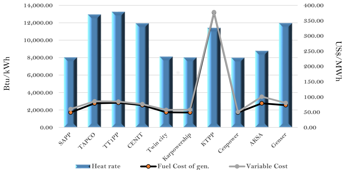
Efficiency and fuel cost of generation on the 28th February 2024
