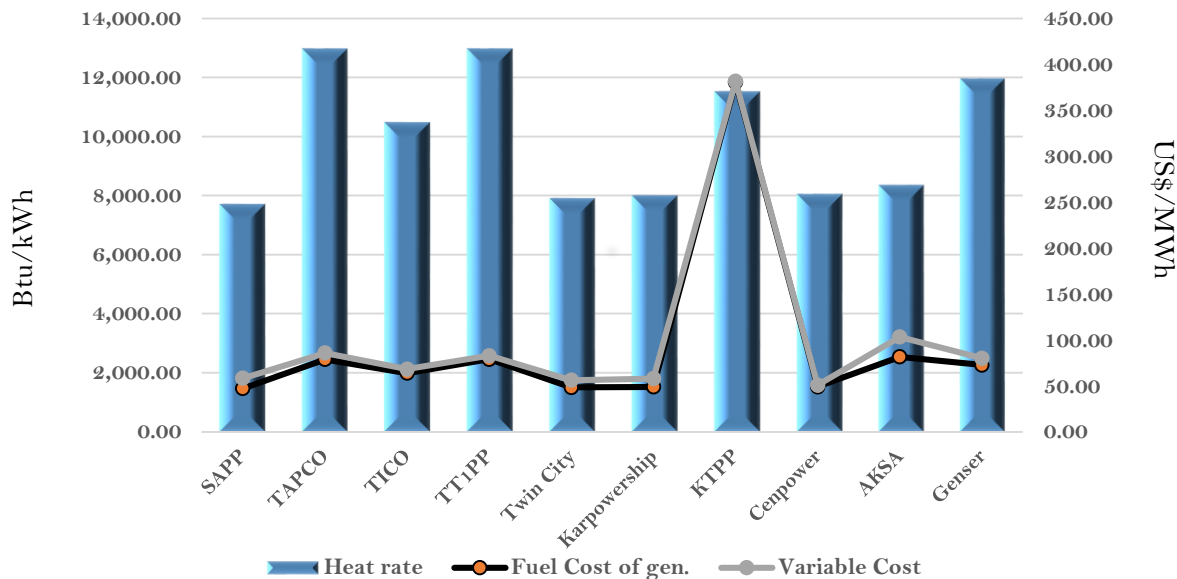
Efficiency and fuel cost of generation on the 24th February 2024
