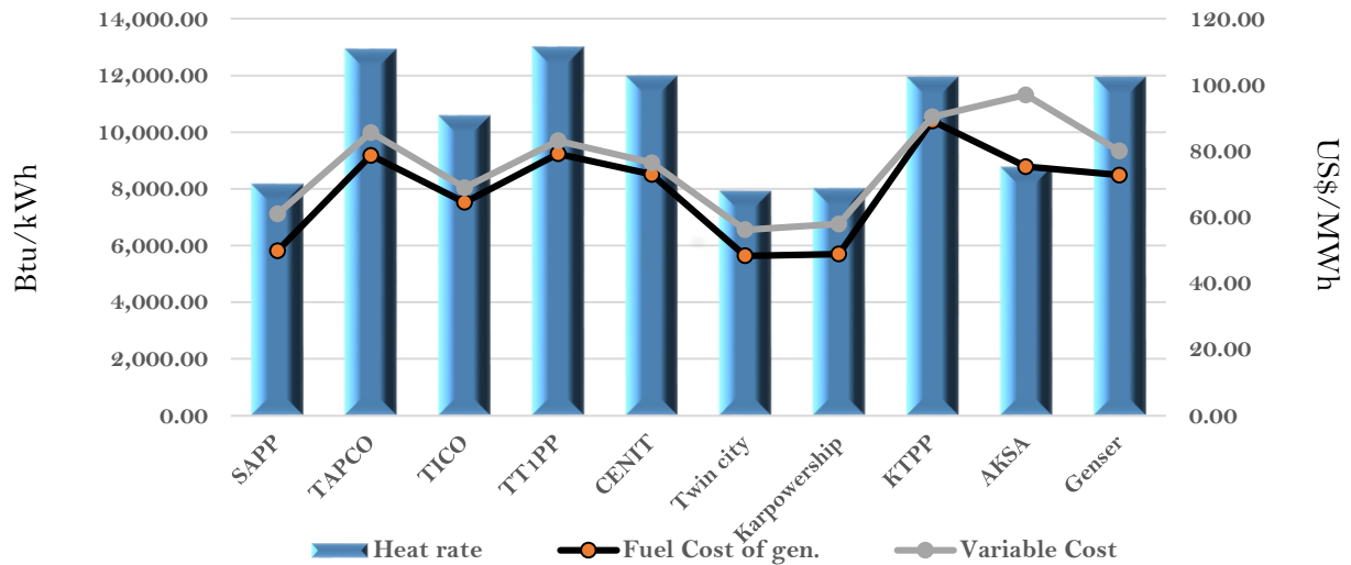
Efficiency and fuel cost of generation on the 29th February 2024
