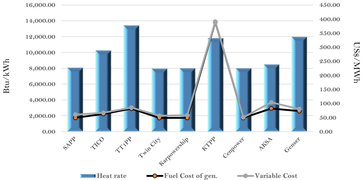
Efficiency and fuel cost of generation on the 26th February 2024
