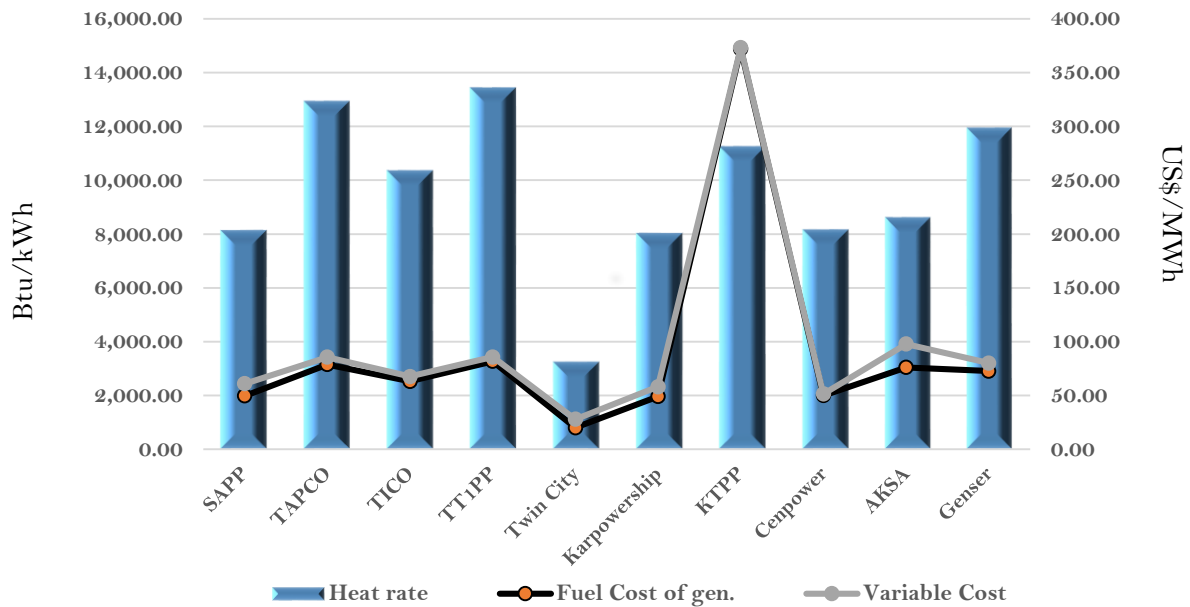
Efficiency and fuel cost of generation on the 27th February 2024
