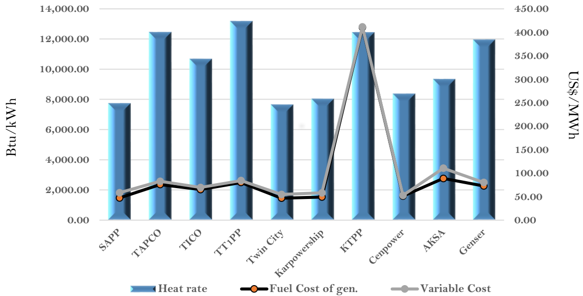
Efficiency and fuel cost of generation on the 23rd February 2024
