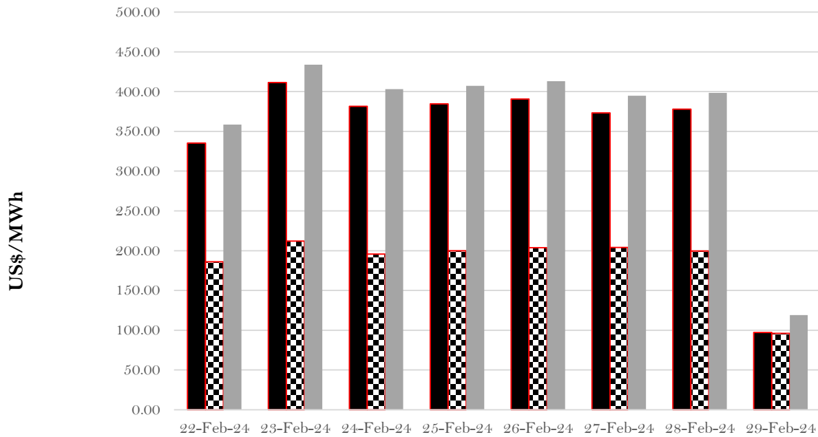
System Marginal Cost Vs Average Market Prices for Week 4 of February 2024
