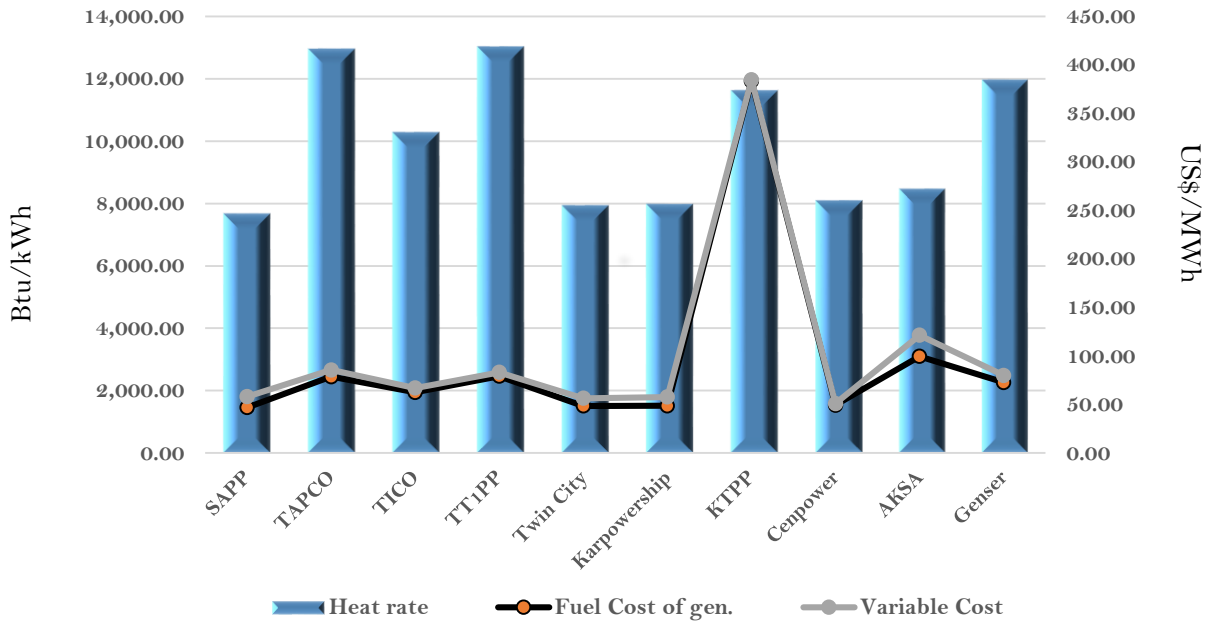
Efficiency and fuel cost of generation on the 26th February 2024
