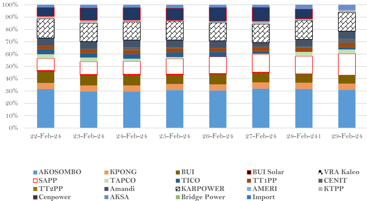
Shares of power plant generation
