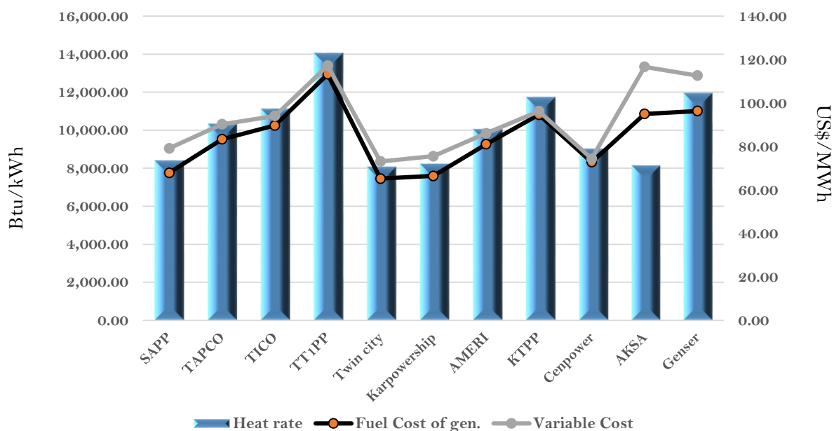
Efficiency and fuel cost of generation on the 17th May 2024
