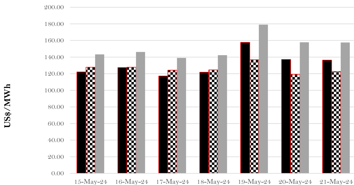
System Marginal Cost Vs Average Market Prices for Week 3 of May 2024
