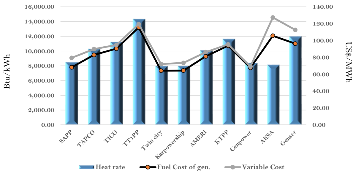
Efficiency and fuel cost of generation on the 17th May 2024
