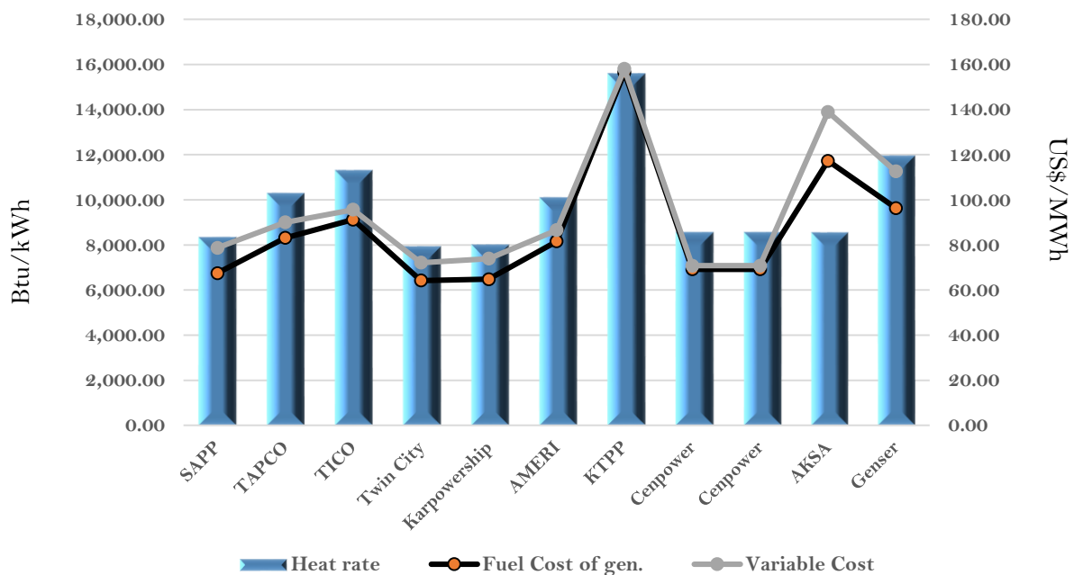
Efficiency and fuel cost of generation on the 19th May 2024
