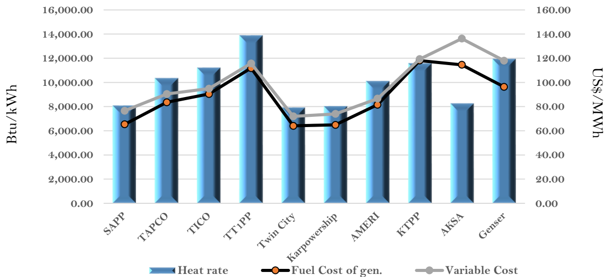
Efficiency and fuel cost of generation on the 21st May 2024
