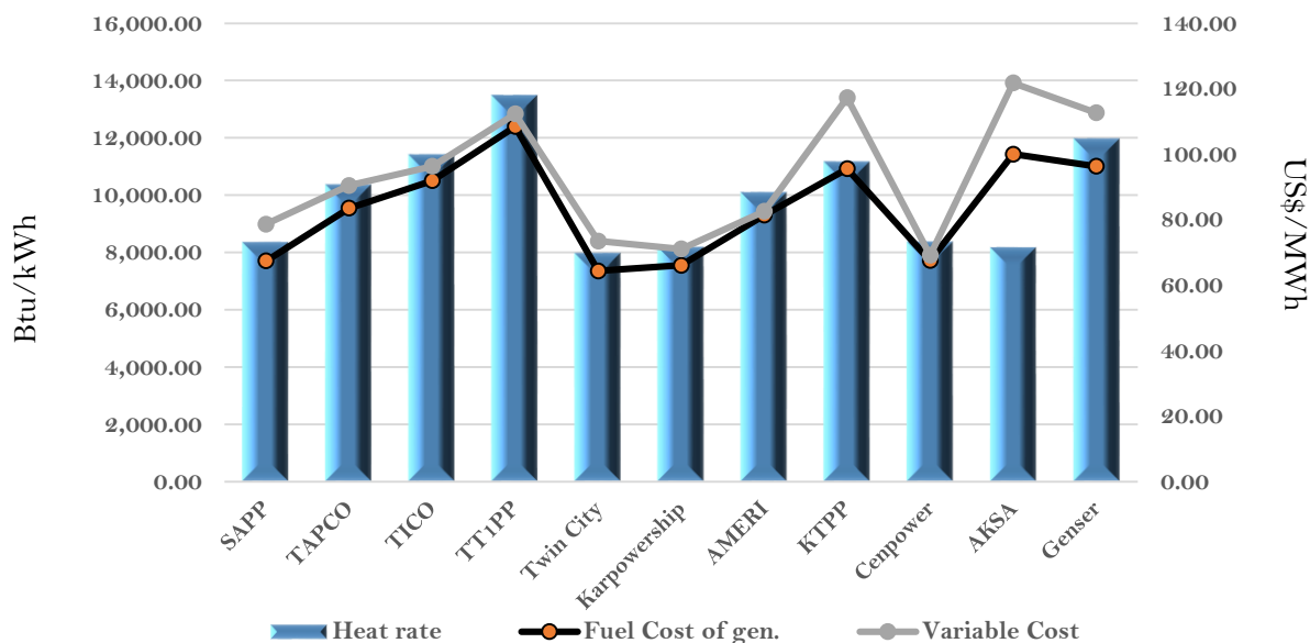
Efficiency and fuel cost of generation on the 18th May 2024
