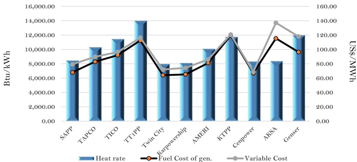
Efficiency and fuel cost of generation on the 20th May 2024
