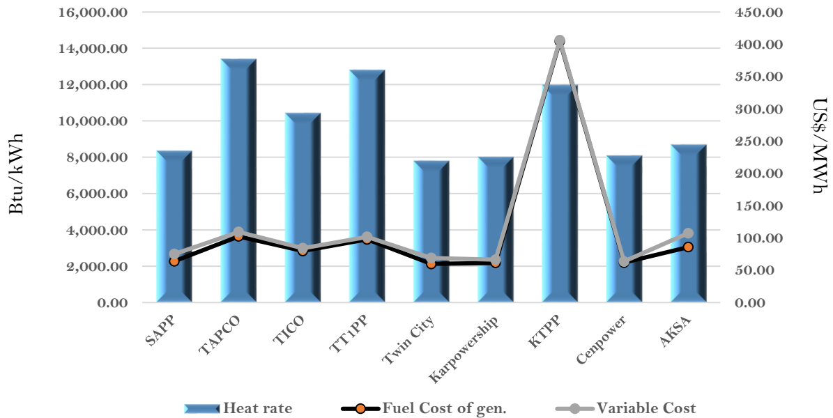
Efficiency and fuel cost of generation on the 19th January 2024
