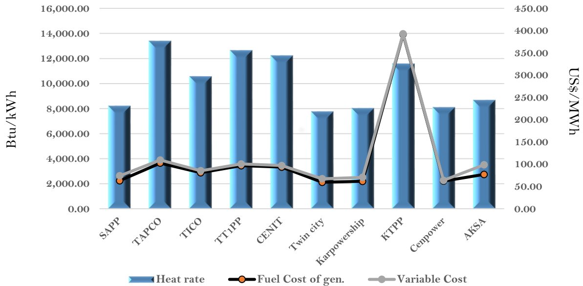
Efficiency and fuel cost of generation on the 16th January 2024
