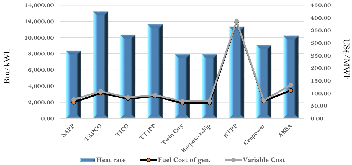
Efficiency and fuel cost of generation on the 20th January 2024
