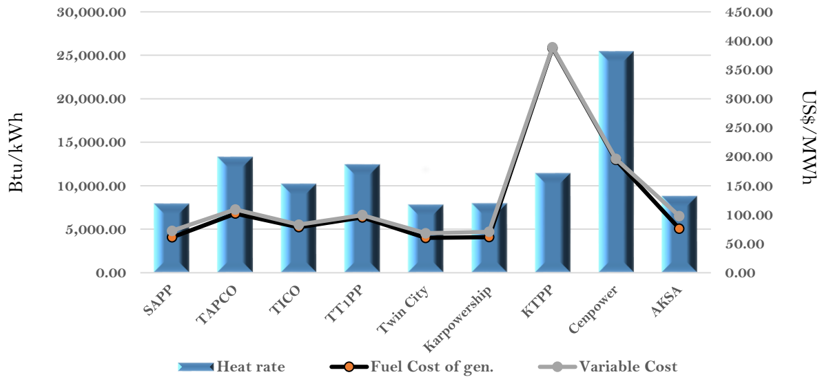
Efficiency and fuel cost of generation on the 21st January 2024
