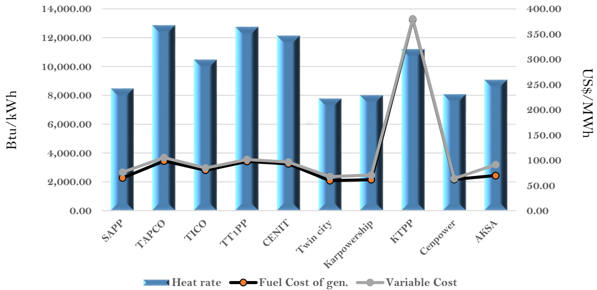
Efficiency and fuel cost of generation on the 17th January 2024
