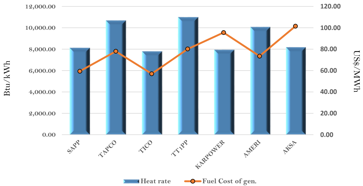
Efficiency and fuel cost of generation on the 9th May 2018
