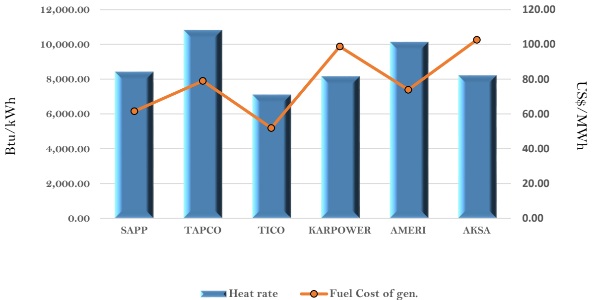
Efficiency and fuel cost of generation on the 13th May 2018
