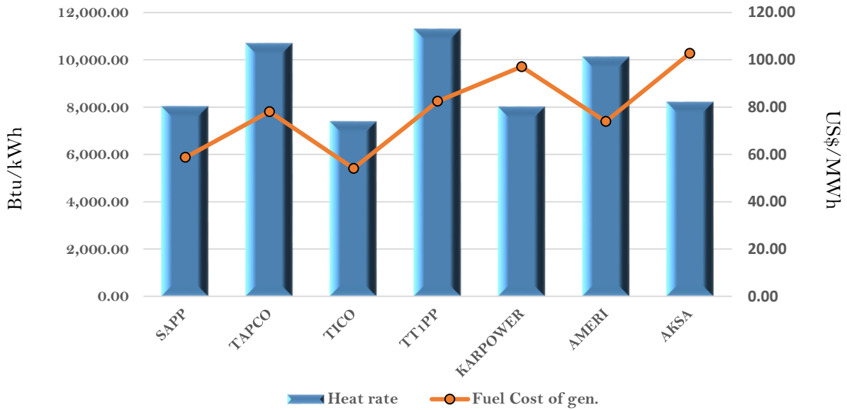
Efficiency and fuel cost of generation on the 12th May 2018
