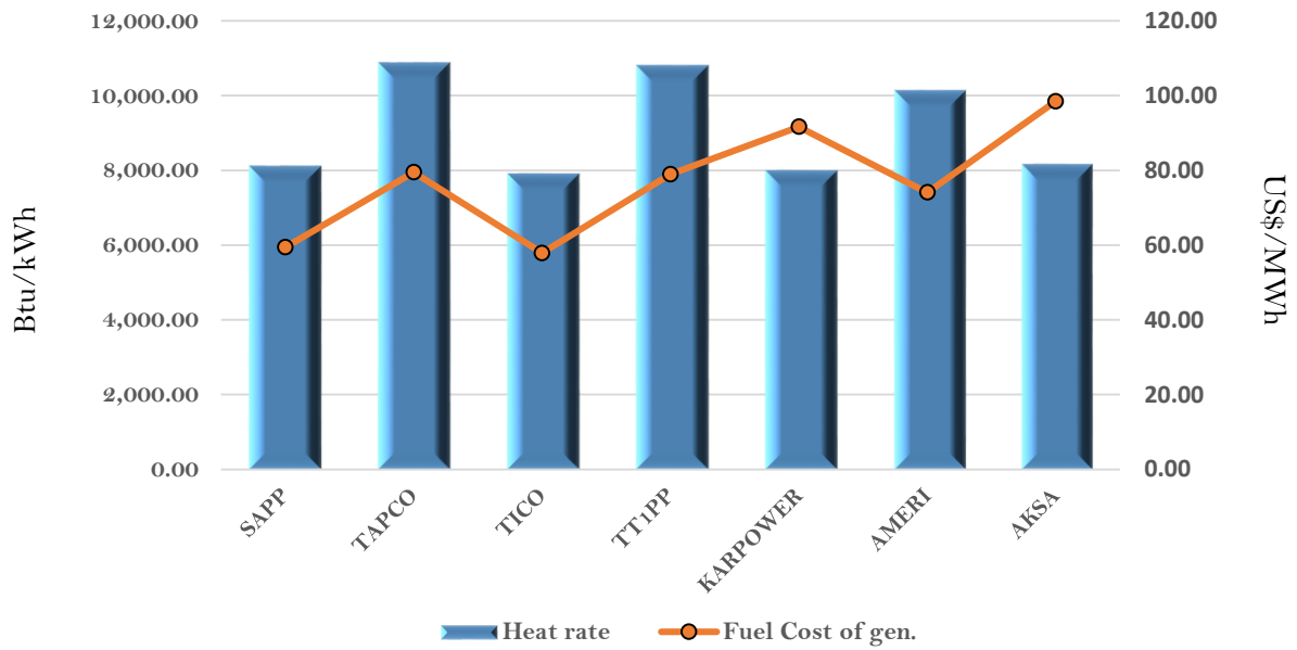
Efficiency and fuel cost of generation on the 9th May 2018
