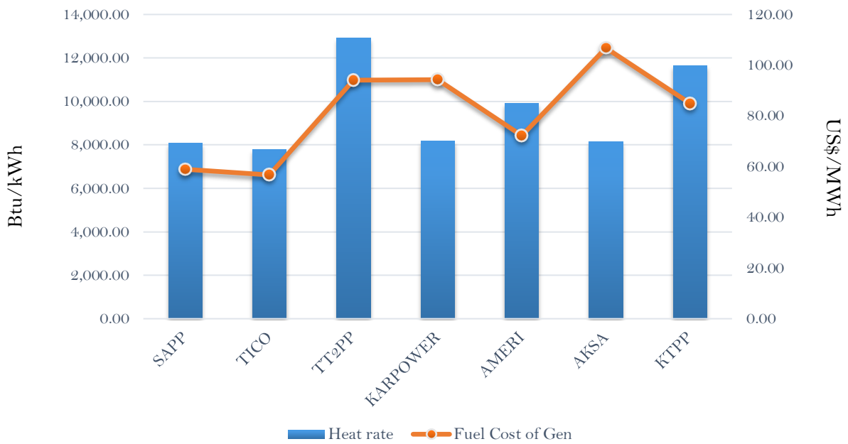
Efficiency and fuel cost of generation on the 20th March 2019
