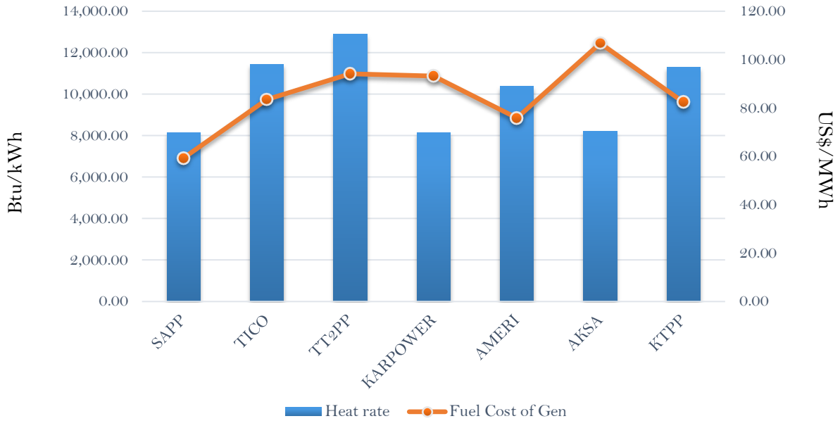
Efficiency and fuel cost of generation on the 16th March 2019
