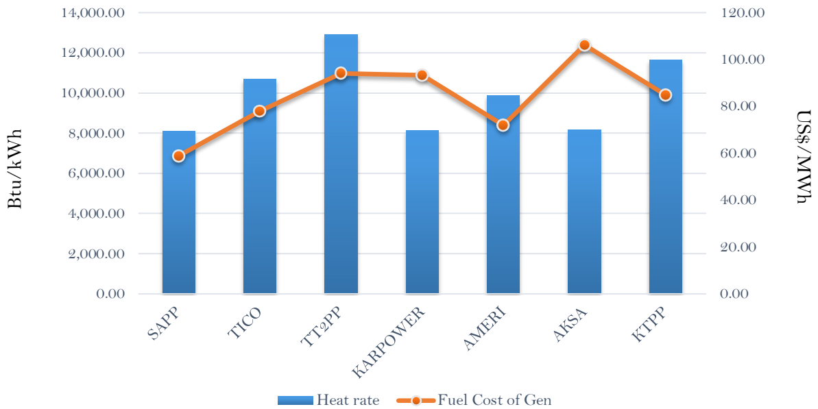
Efficiency and fuel cost of generation on the 19th March 2019
