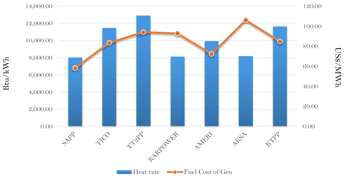
Efficiency and fuel cost of generation on the 18th March 2019
