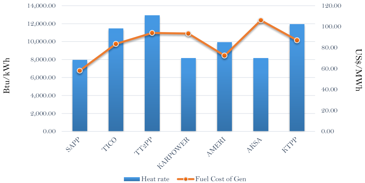
Efficiency and fuel cost of generation on the 18th March 2019
