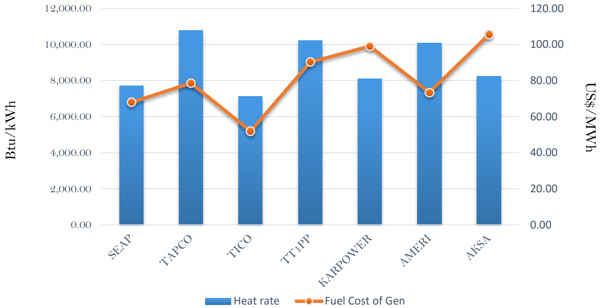
Efficiency and fuel cost of generation on the 5th July 2018
