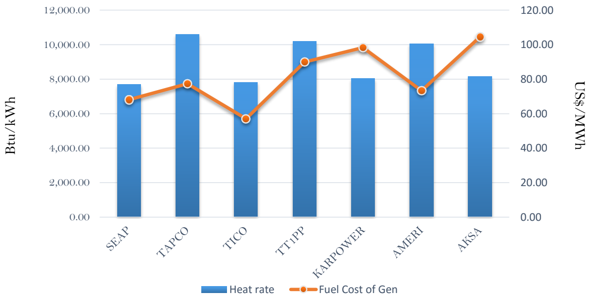
Efficiency and fuel cost of generation on the 6th July 2018
