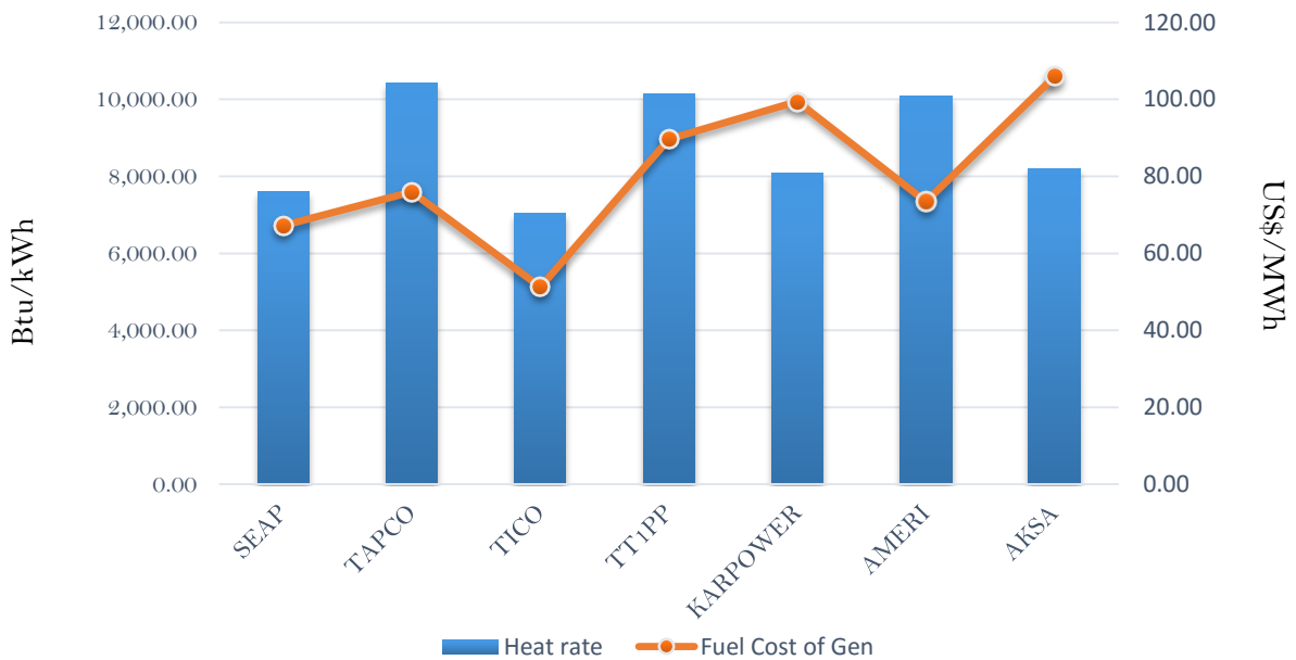
Efficiency and fuel cost of generation on the 4th July 2018
