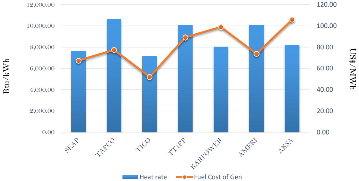
Efficiency and fuel cost of generation on the 3rd July 2018
