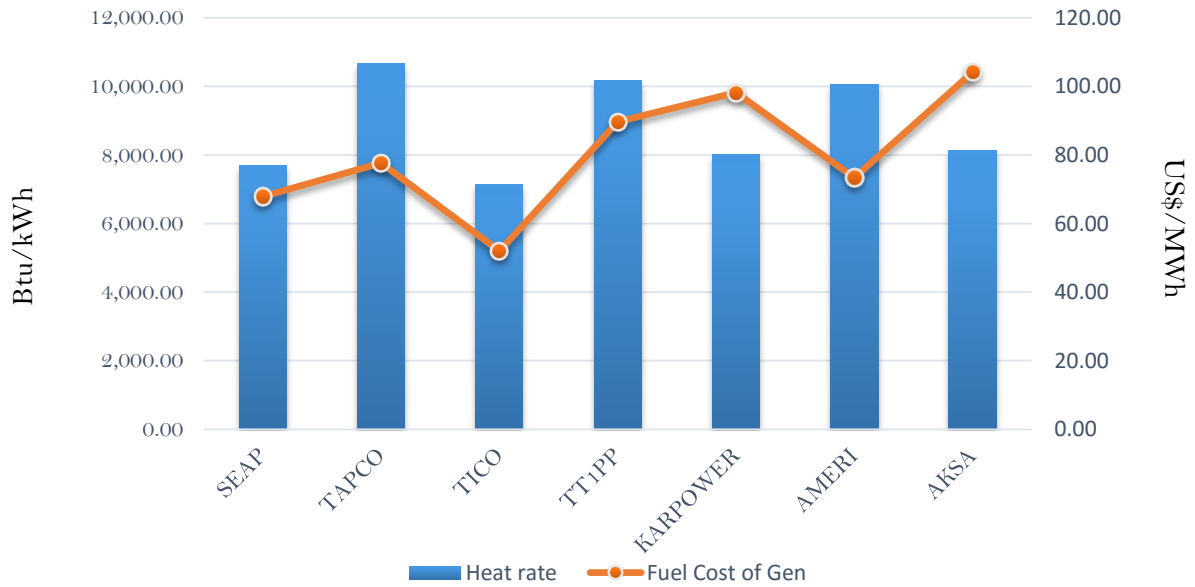
Efficiency and fuel cost of generation on the 2nd July 2018
