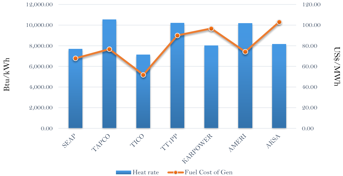
Efficiency and fuel cost of generation on the 1st July 2018
