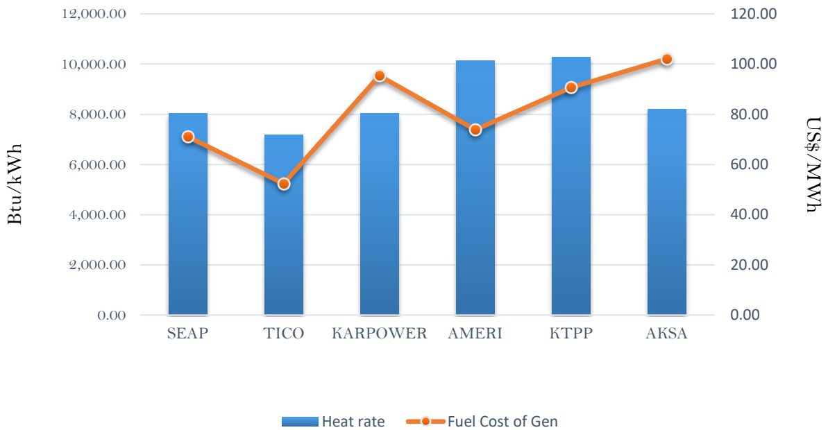
Efficiency and fuel cost of generation on the 23rd August 2018
