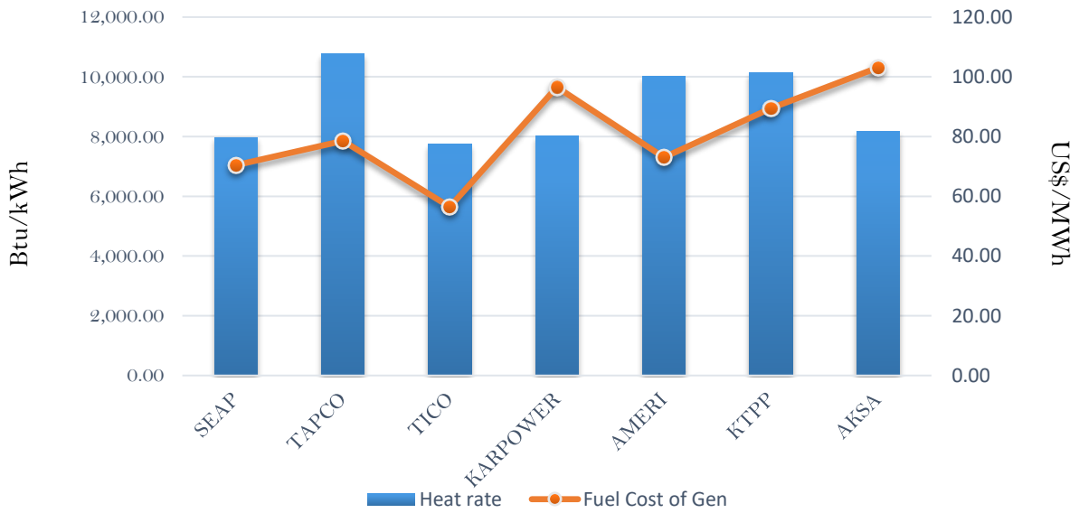
Efficiency and fuel cost of generation on the 31st August 2018
