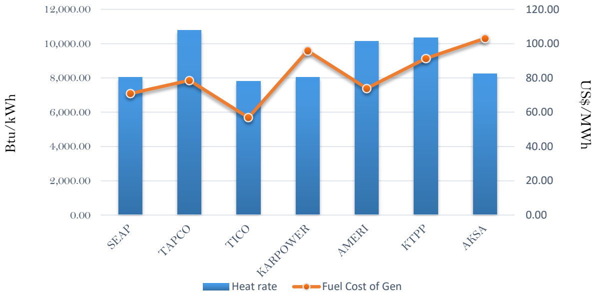
Efficiency and fuel cost of generation on the 28th August 2018
