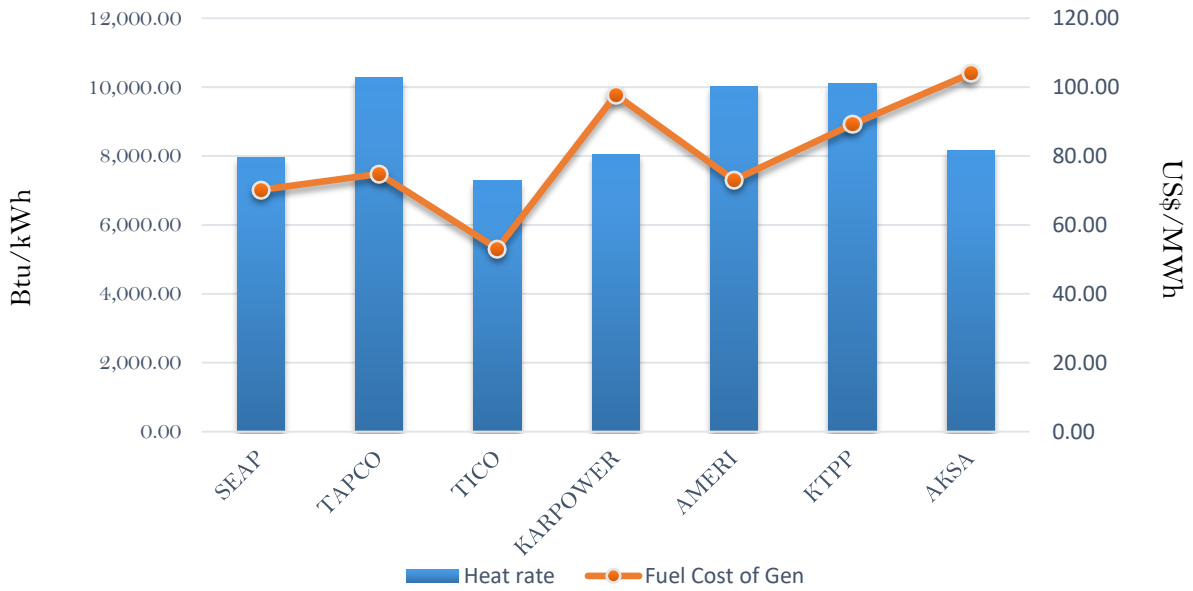
Efficiency and fuel cost of generation on the 30th August 2018
