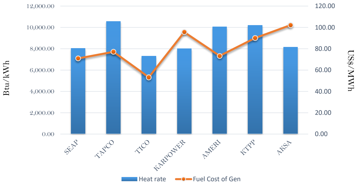
Efficiency and fuel cost of generation on the 25th August 2018
