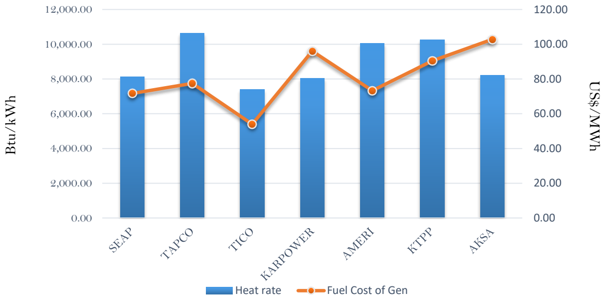
Efficiency and fuel cost of generation on the 26th August 2018
