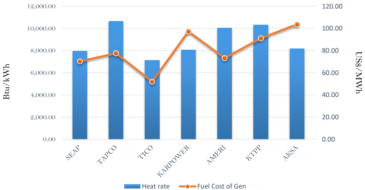
Efficiency and fuel cost of generation on the 29th August 2018
