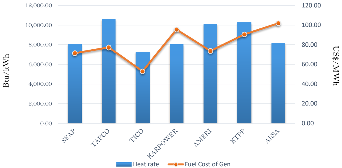
Efficiency and fuel cost of generation on the 22nd August 2018
