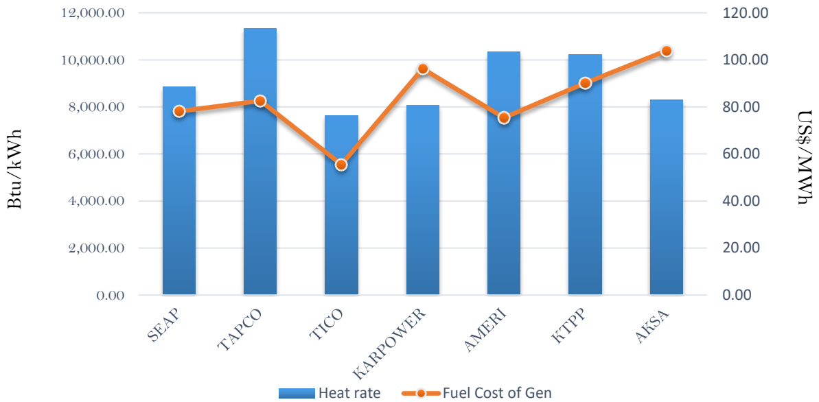
Efficiency and fuel cost of generation on the 24th August 2018
