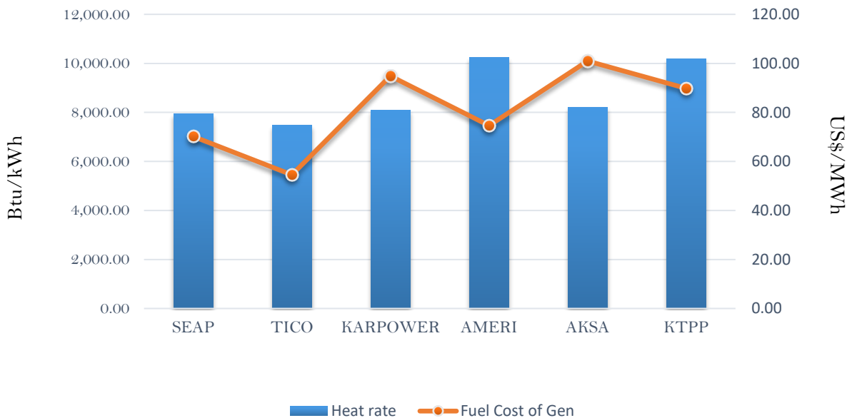
Efficiency and fuel cost of generation on the 9th August 2018
