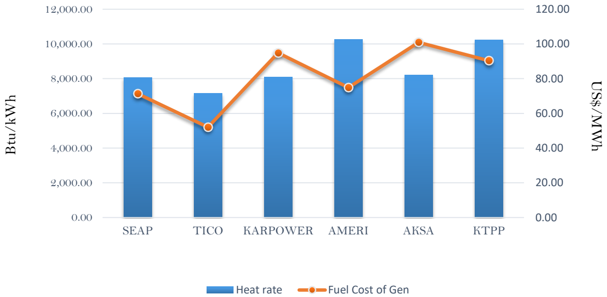
Efficiency and fuel cost of generation on the 8th August 2018
