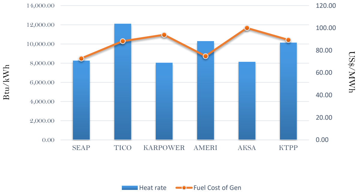
Efficiency and fuel cost of generation on the 13th August 2018
