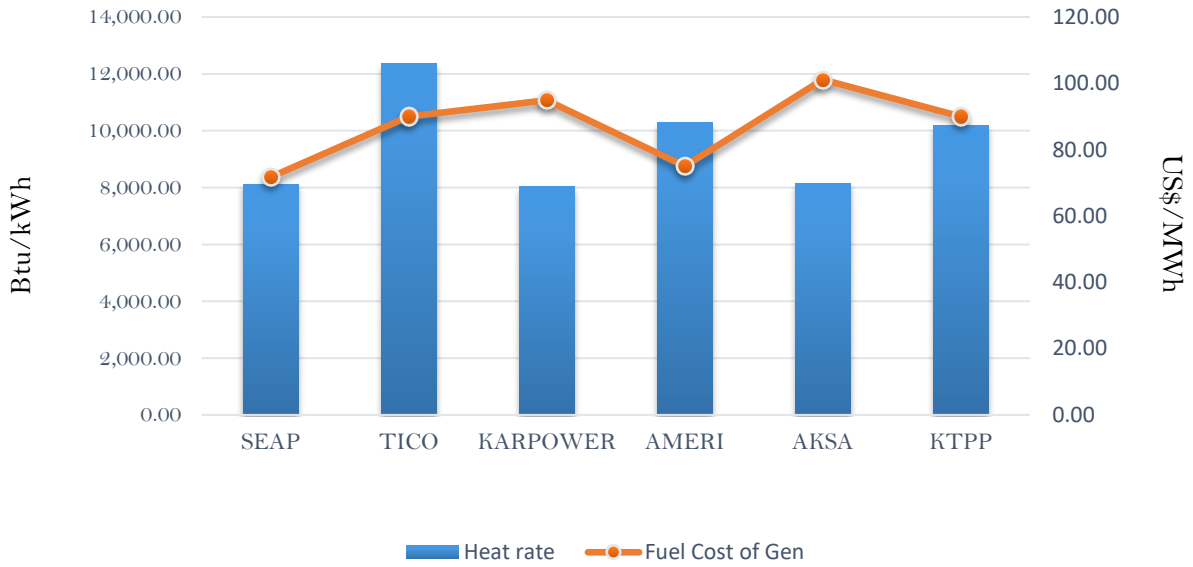
Efficiency and fuel cost of generation on the 12th August 2018
