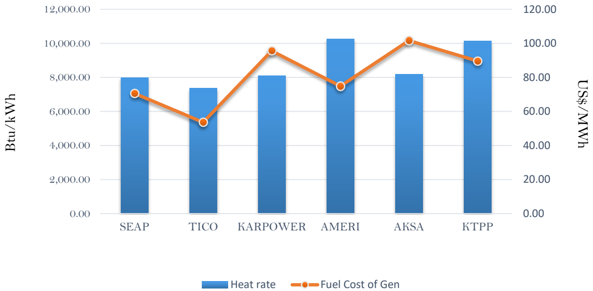
Efficiency and fuel cost of generation on the 10th August 2018
