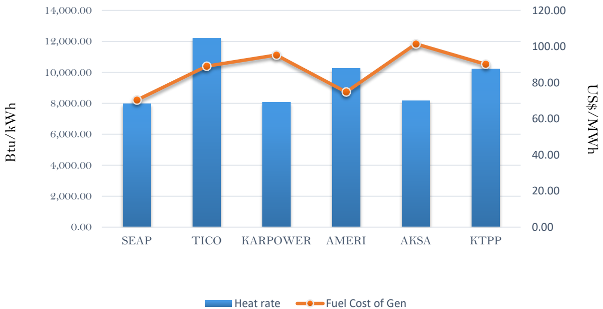
Efficiency and fuel cost of generation on the 11th August 2018
