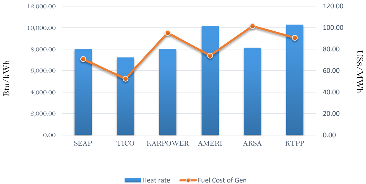
Efficiency and fuel cost of generation on the 6th August 2018
