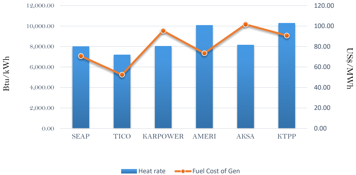
Efficiency and fuel cost of generation on the 5th August 2018
