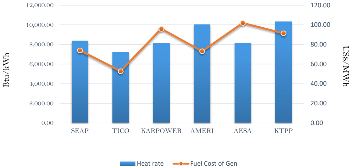
Efficiency and fuel cost of generation on the 3rd August 2018
