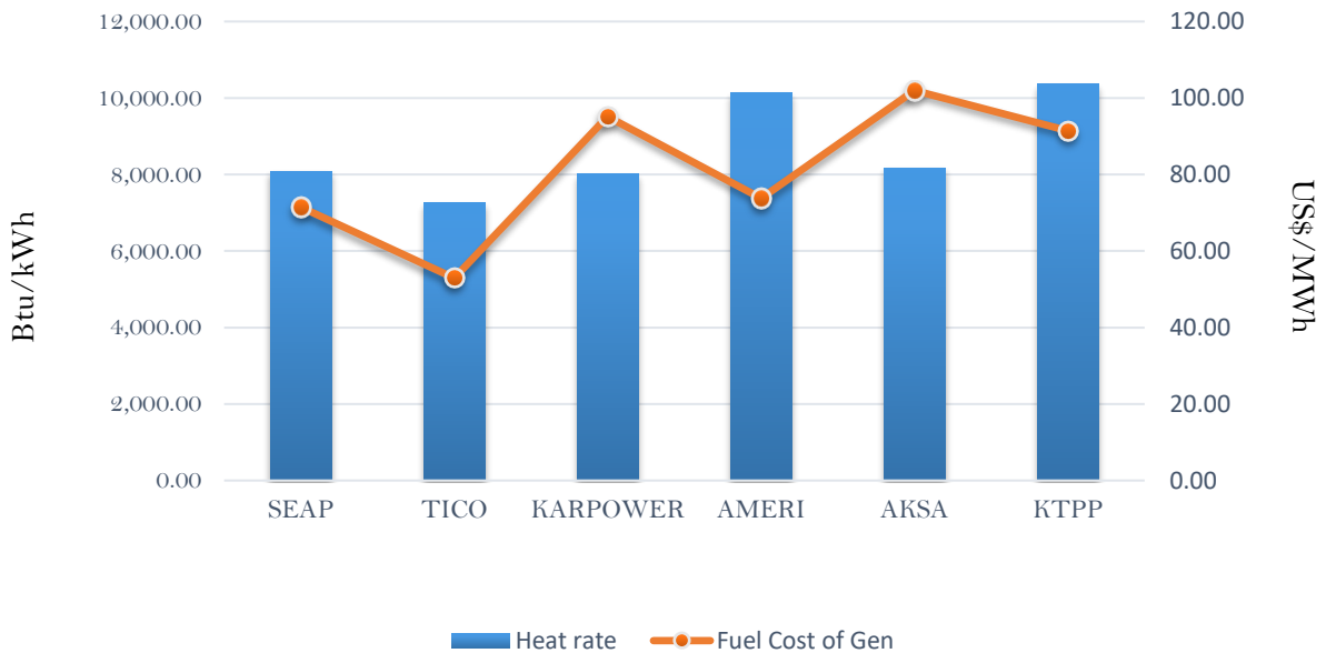
Efficiency and fuel cost of generation on the 4th August 2018
