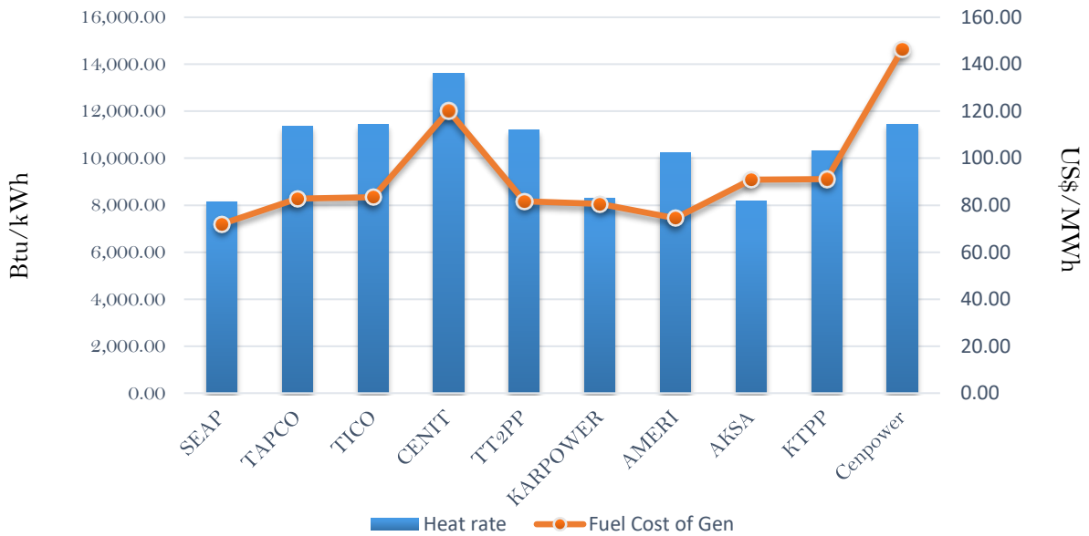
Efficiency and fuel cost of generation on the 17th December 2018
