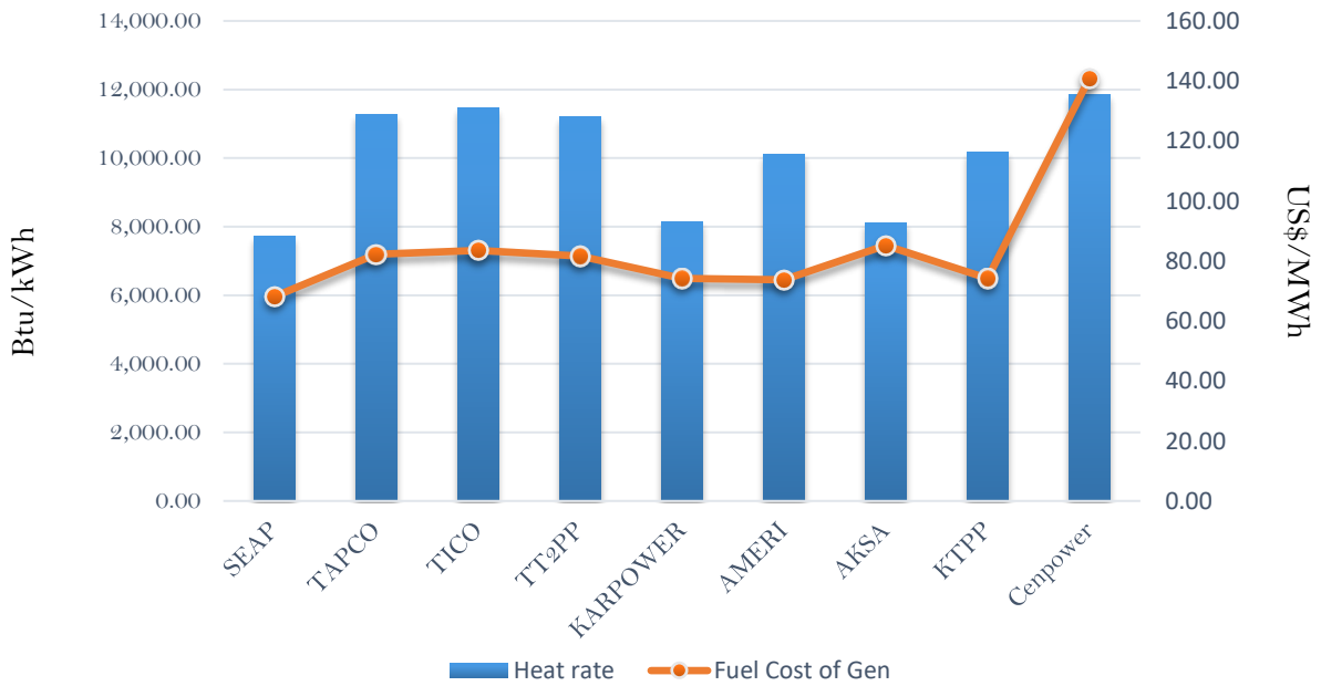
Efficiency and fuel cost of generation on the 20th December 2018
