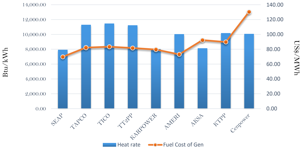
Efficiency and fuel cost of generation on the 15th December 2018
