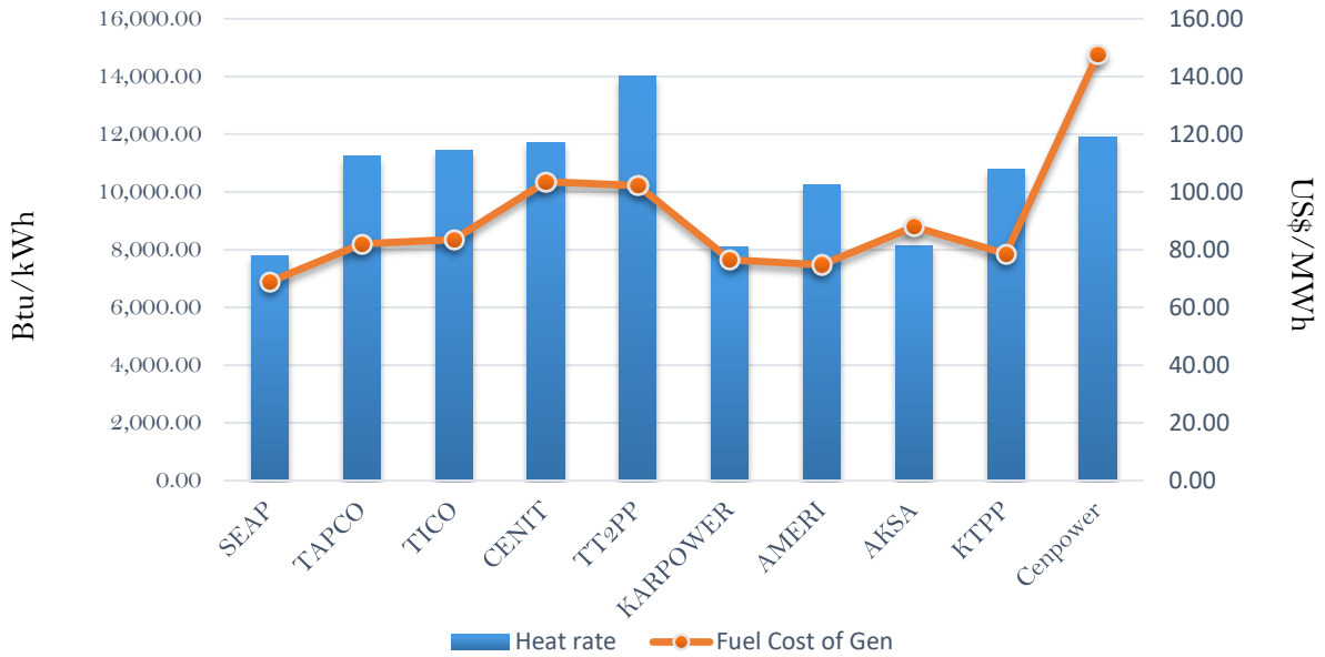
Efficiency and fuel cost of generation on the 19th December 2018
