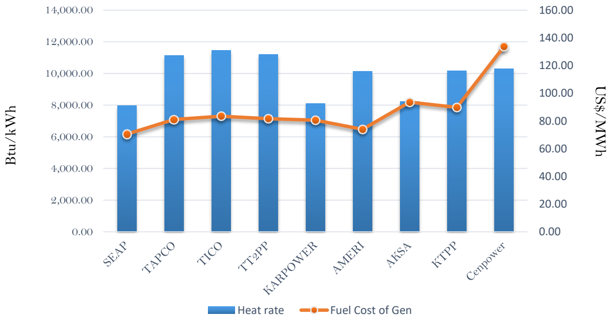
Efficiency and fuel cost of generation on the 16th December 2018
