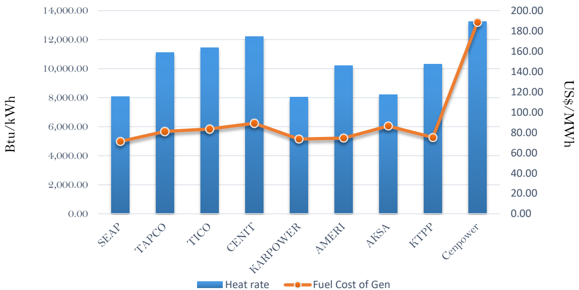
Efficiency and fuel cost of generation on the 18th December 2018
