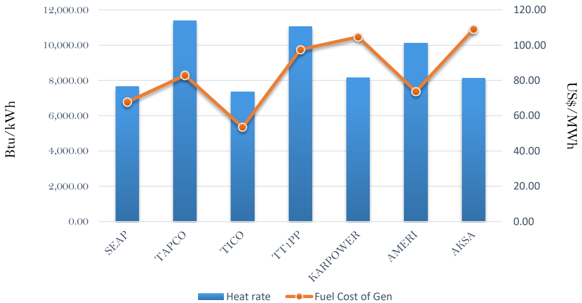
Efficiency and fuel cost of generation on the 29th September 2018
