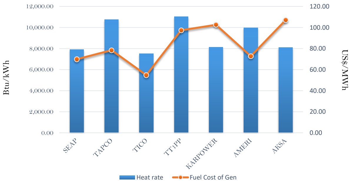
Efficiency and fuel cost of generation on the 25th September 2018
