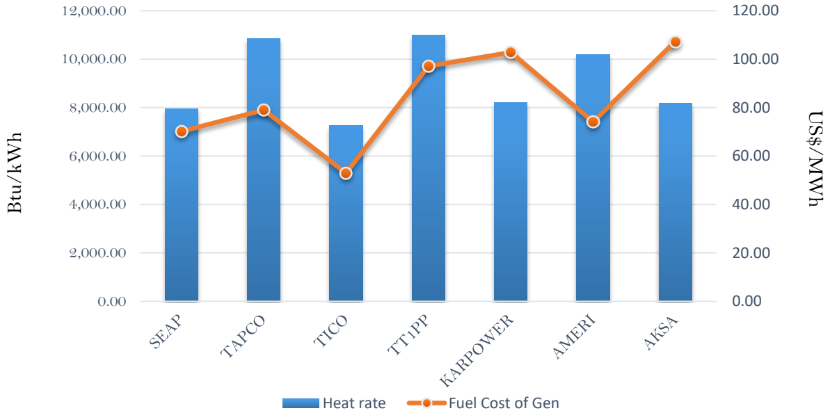
Efficiency and fuel cost of generation on the 26th September 2018
