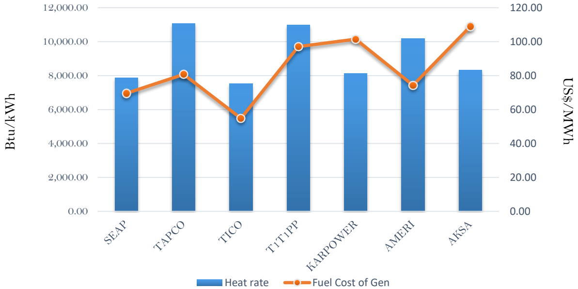
Efficiency and fuel cost of generation on the 24th September 2018
