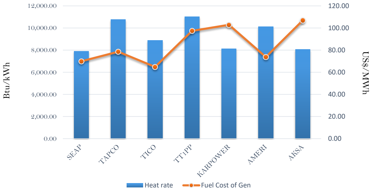
Efficiency and fuel cost of generation on the 27th September 2018
