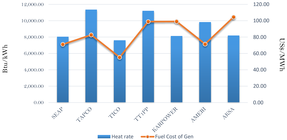
Efficiency and fuel cost of generation on the 22nd September 2018
