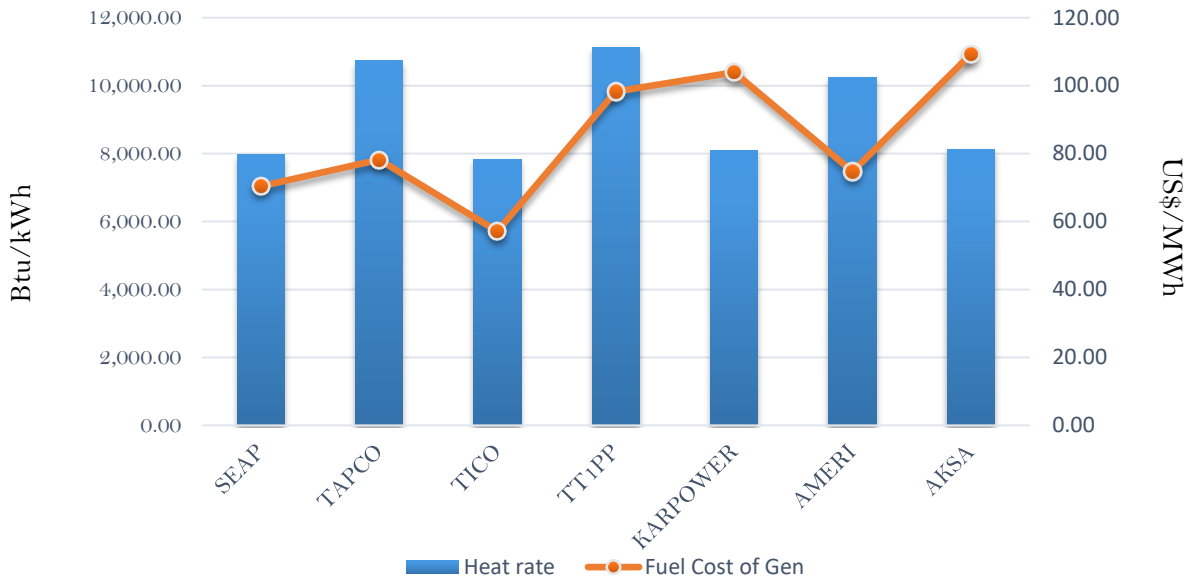
Efficiency and fuel cost of generation on the 28th September 2018
