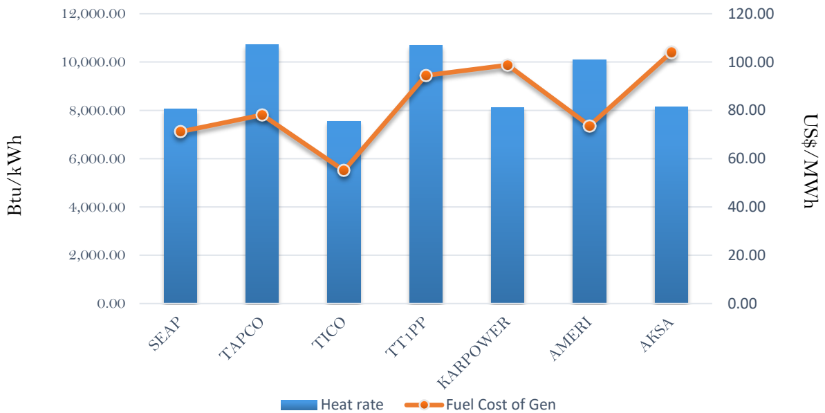
Efficiency and fuel cost of generation on the 23rd September 2018
