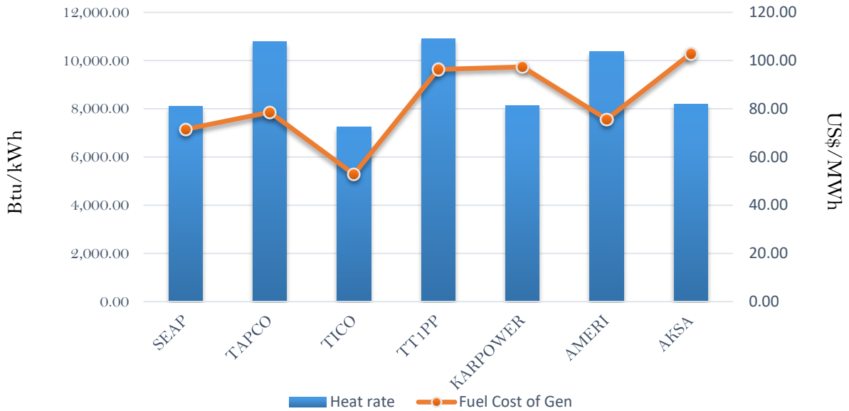
Efficiency and fuel cost of generation on 10th September 2018
