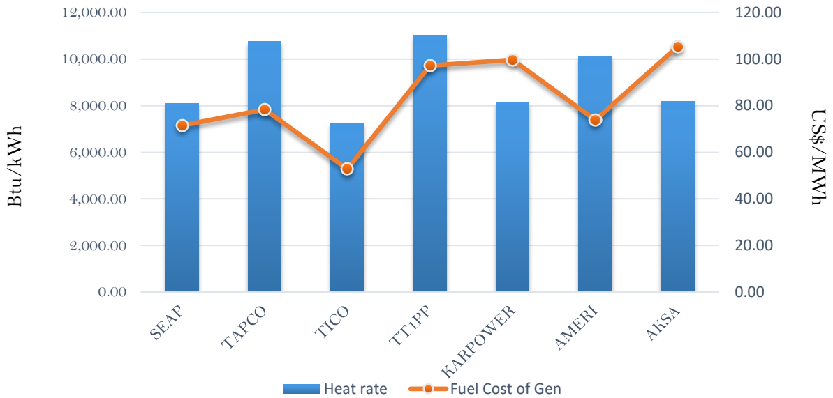
Efficiency and fuel cost of generation on 12th September 2018
