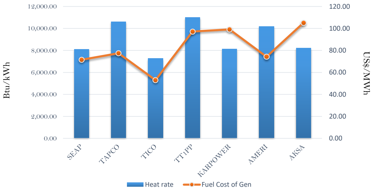
Efficiency and fuel cost of generation on 11th September 2018
