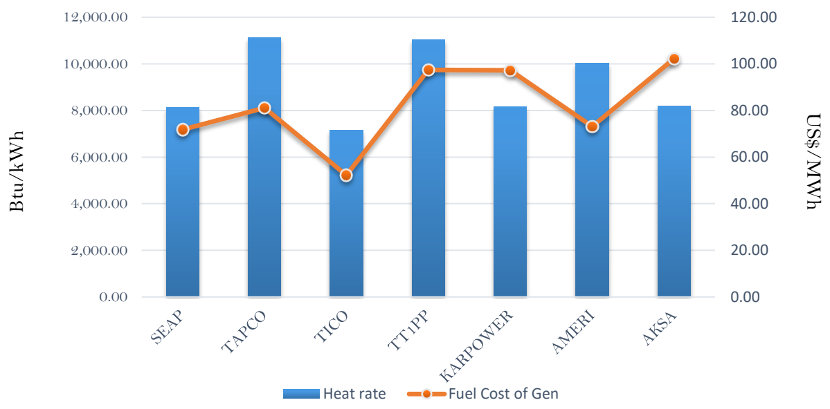
Efficiency and fuel cost of generation on 8th September 2018
