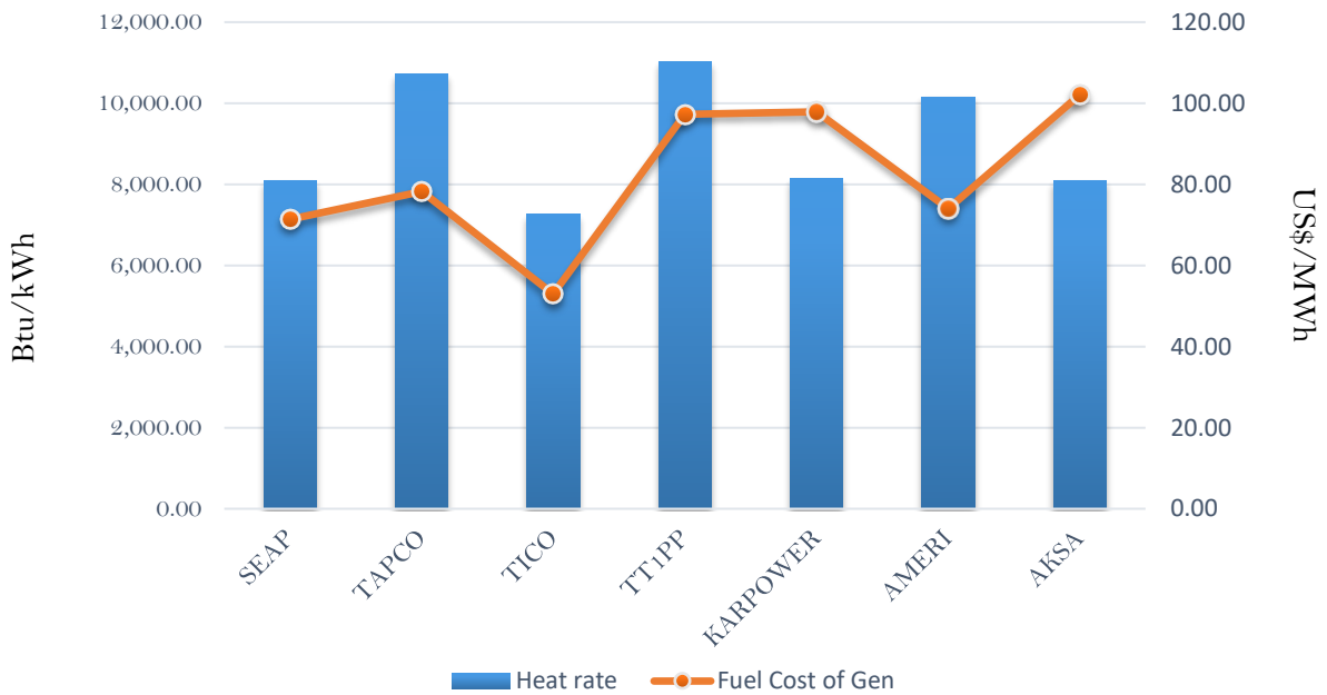
Efficiency and fuel cost of generation on 13th September 2018
