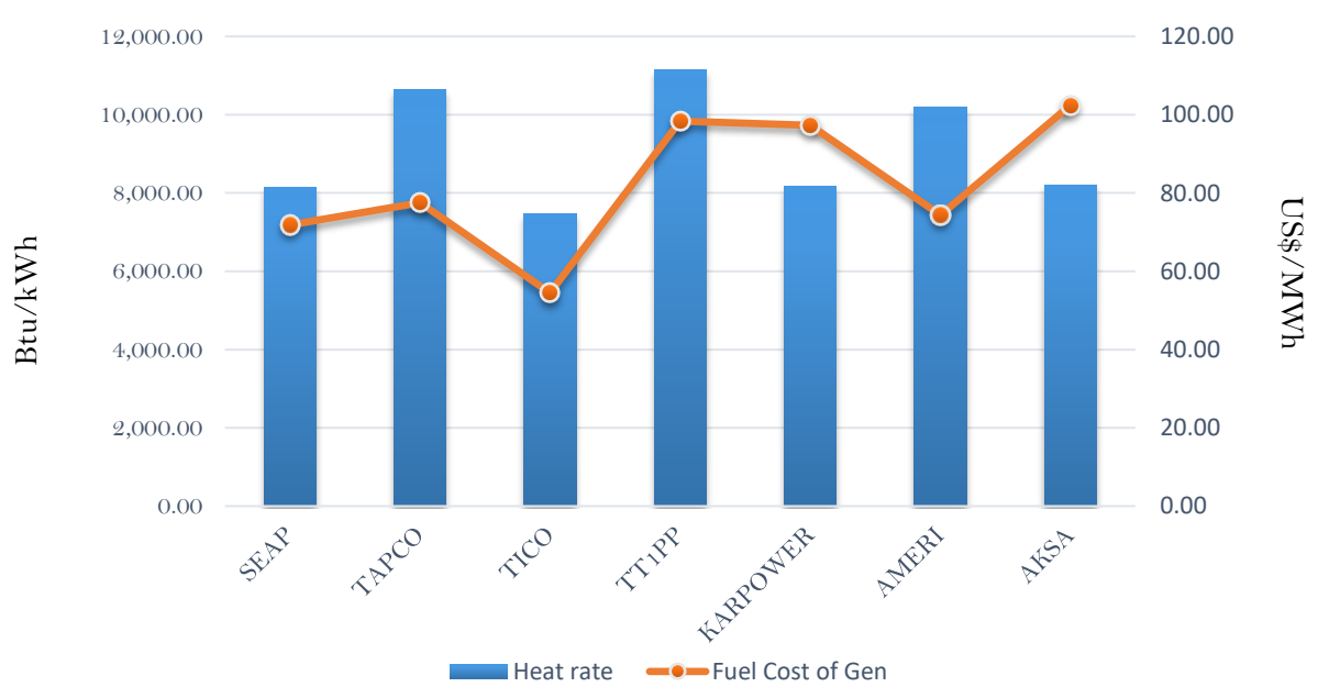
Efficiency and fuel cost of generation on 9th September 2018
