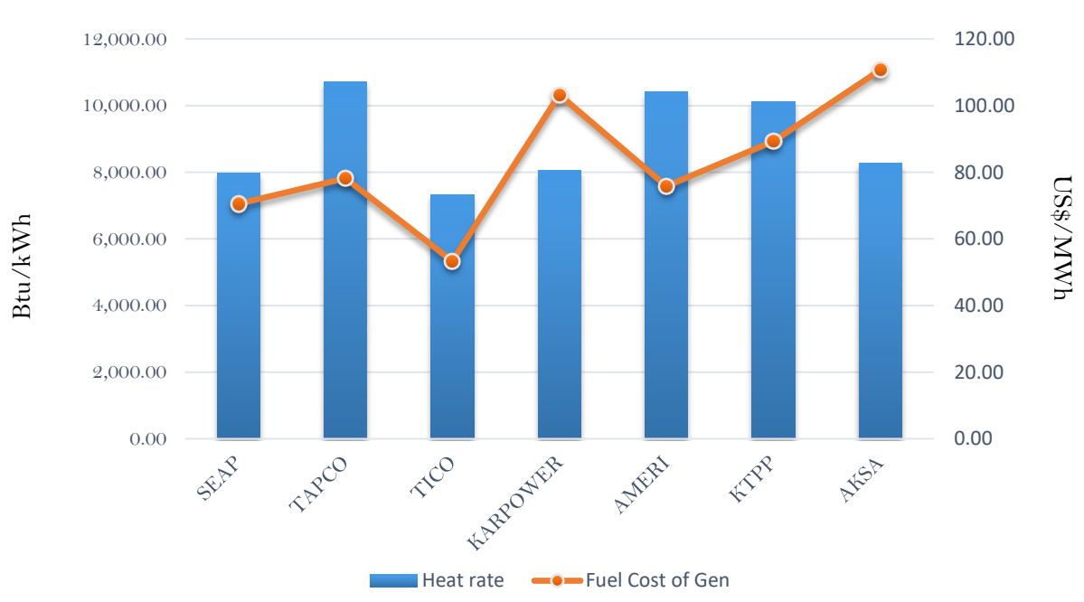
Efficiency and fuel cost of generation on the 29th October 2018
