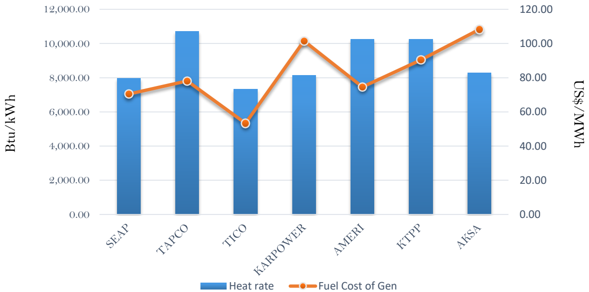
Efficiency and fuel cost of generation on the 23rd October 2018
