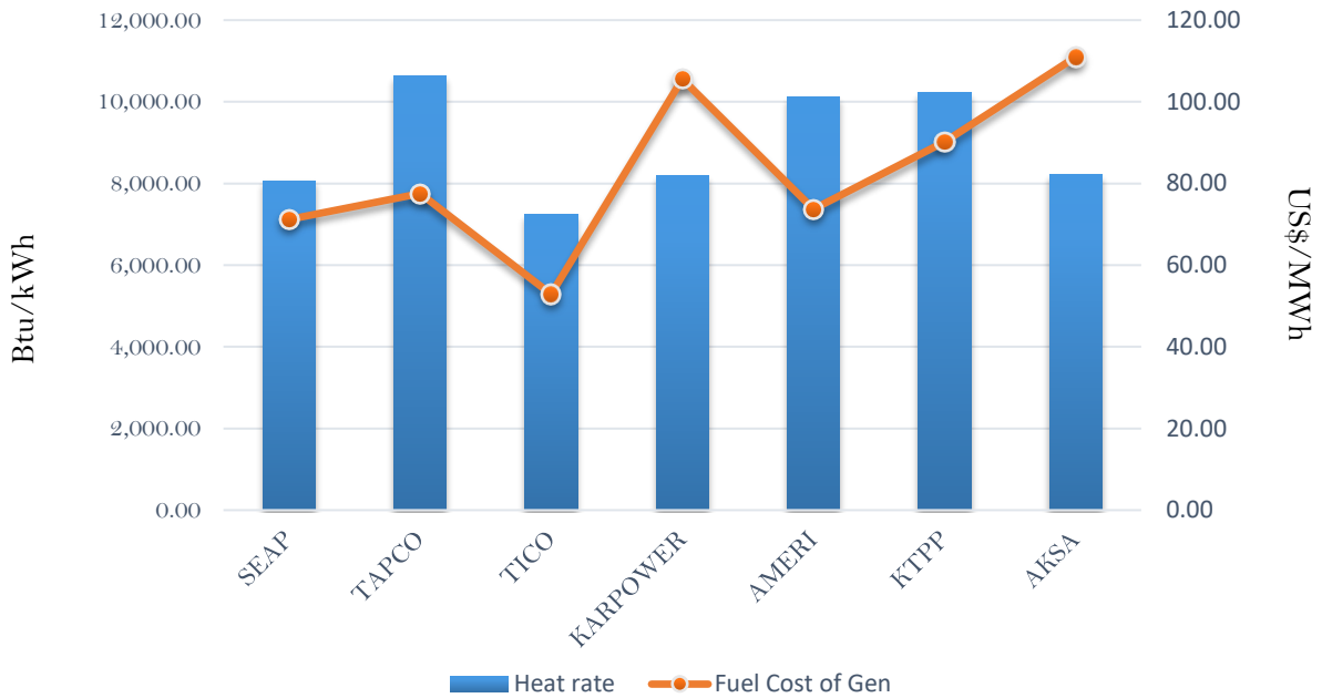
Efficiency and fuel cost of generation on the 27th October 2018
