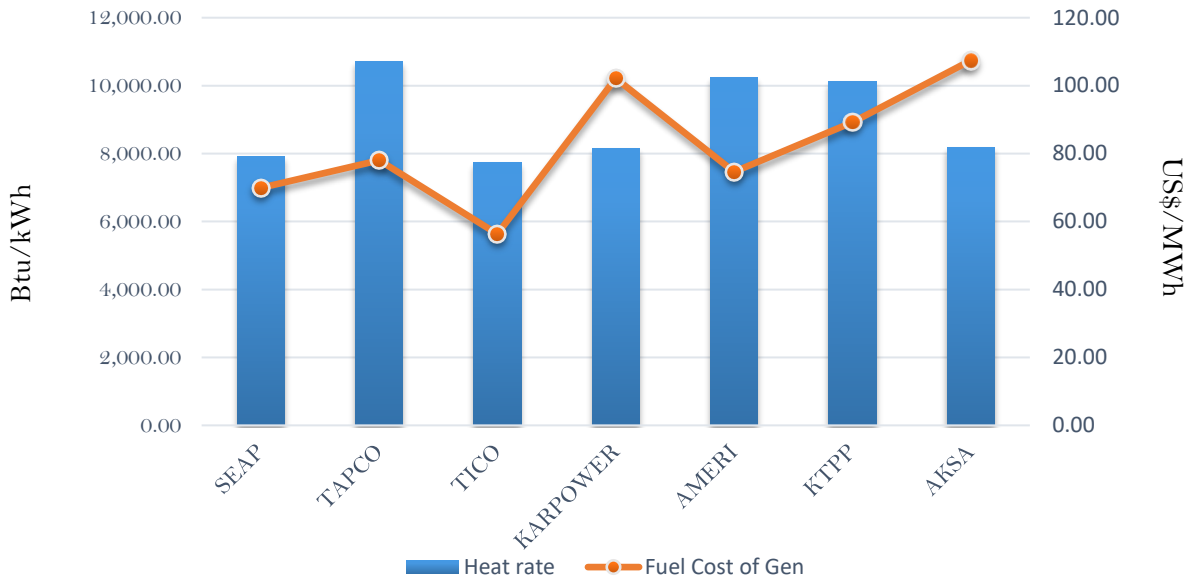
Efficiency and fuel cost of generation on the 24th October 2018
