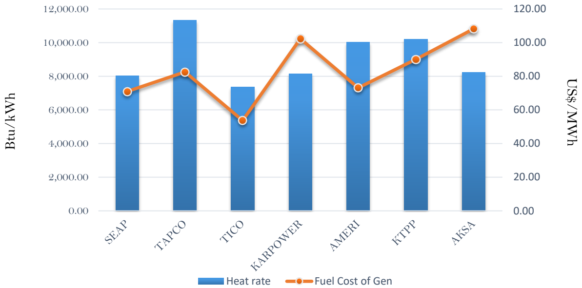
Efficiency and fuel cost of generation on the 30th October 2018
