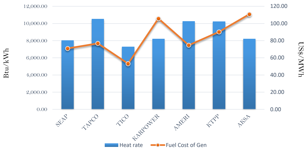
Efficiency and fuel cost of generation on the 28th October 2018
