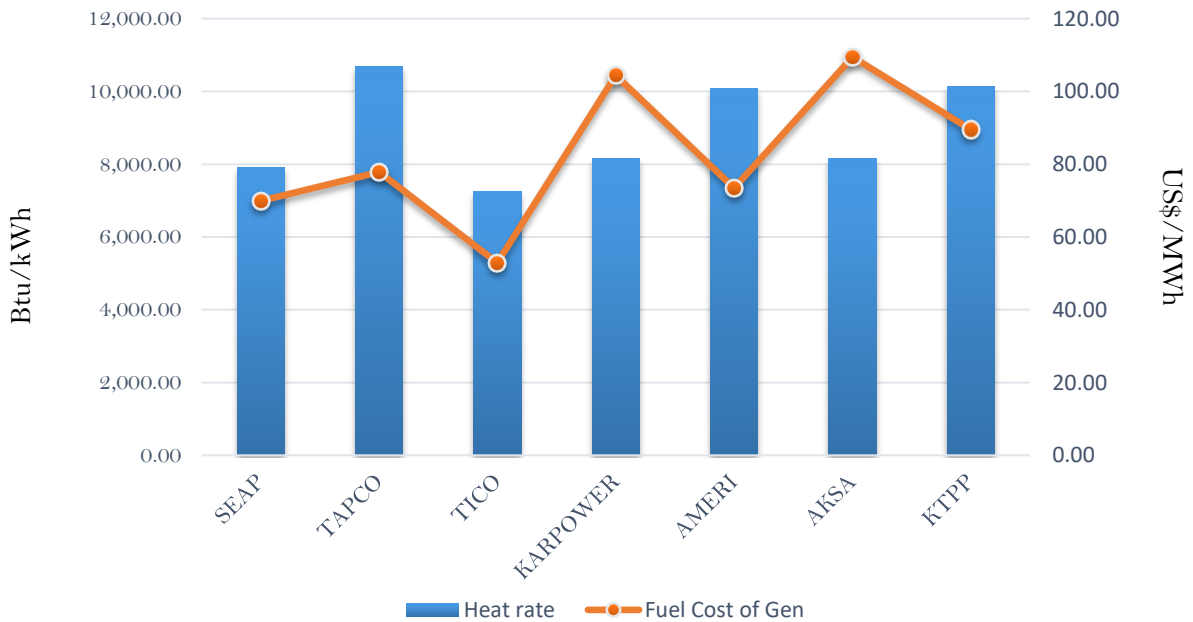
Efficiency and fuel cost of generation on the 25th October 2018
