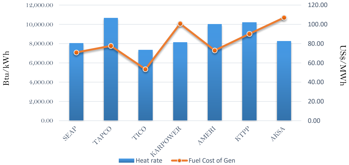
Efficiency and fuel cost of generation on the 31st October 2018
