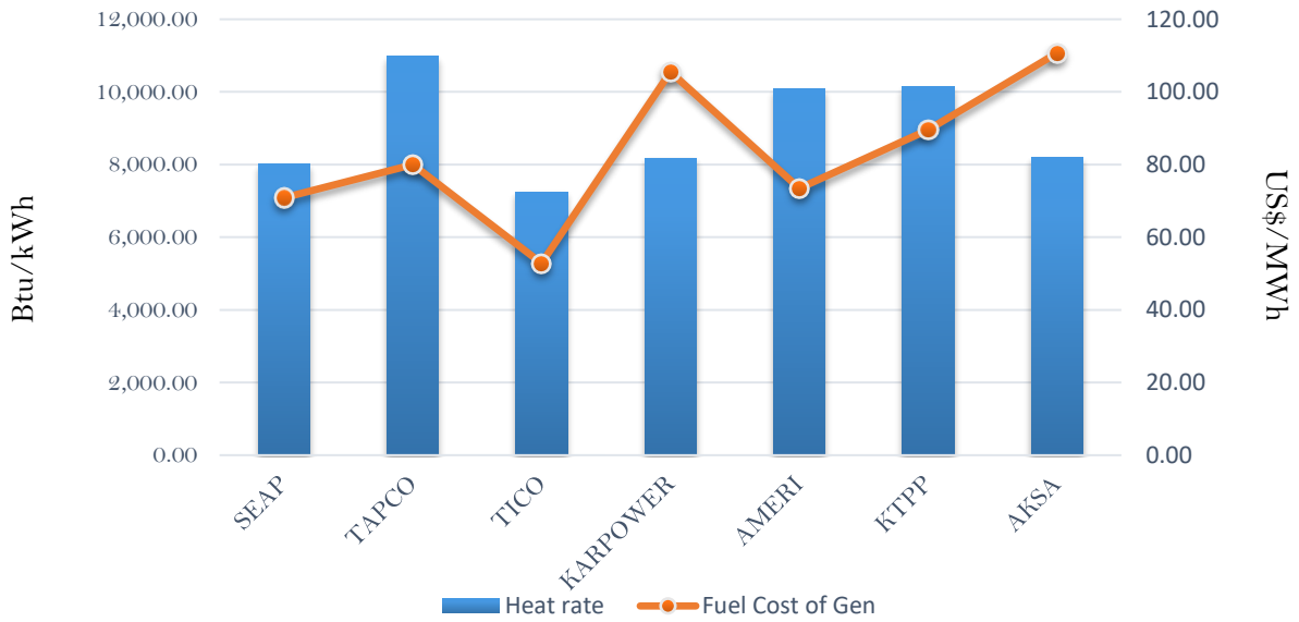
Efficiency and fuel cost of generation on the 26th October 2018
