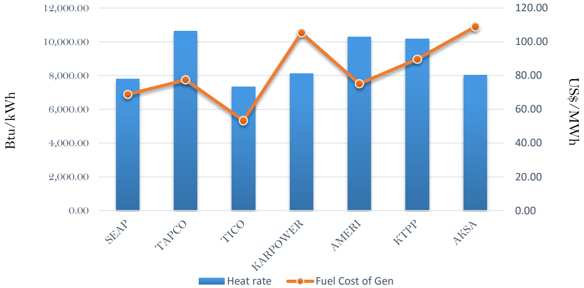
Efficiency and fuel cost of generation on the 22nd October 2018
