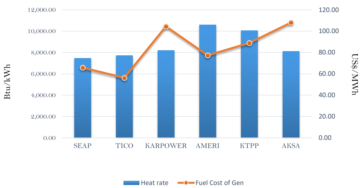
Efficiency and fuel cost of generation on the 11th October 2018
