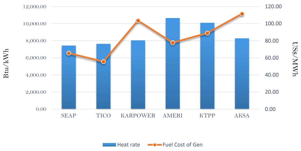
Efficiency and fuel cost of generation on the 12th October 2018
