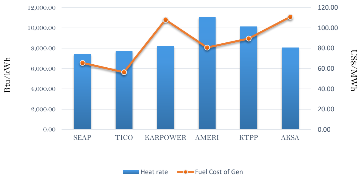
Efficiency and fuel cost of generation on the 10th October 2018
