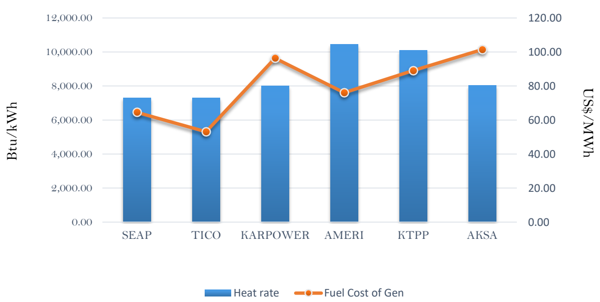
Efficiency and fuel cost of generation on the 13th October 2018
