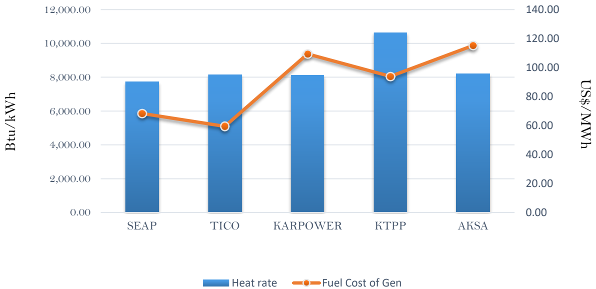
Efficiency and fuel cost of generation on the 3rd October 2018
