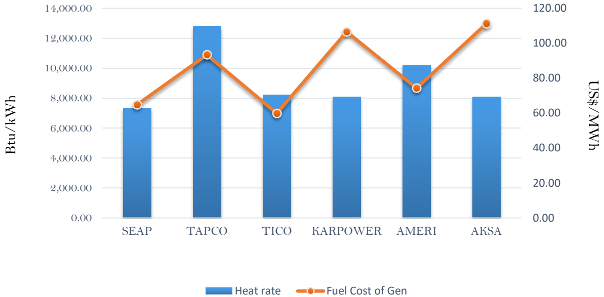
Efficiency and fuel cost of generation on the 1st October 2018
