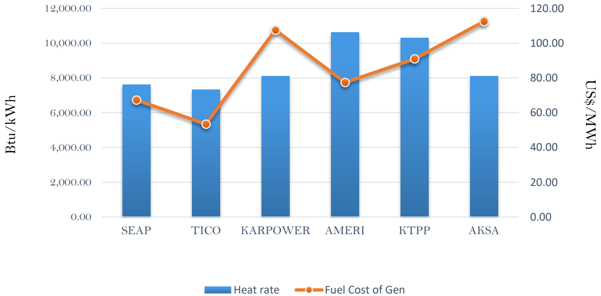
Efficiency and fuel cost of generation on the 5th October 2018
