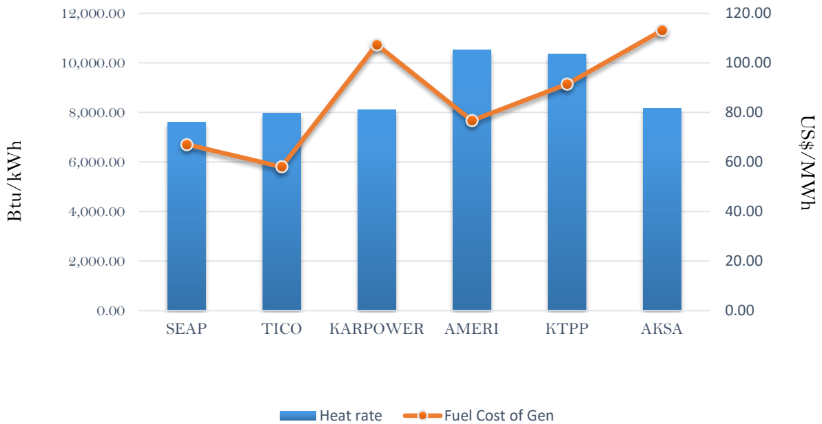
Efficiency and fuel cost of generation on the 4th October 2018
