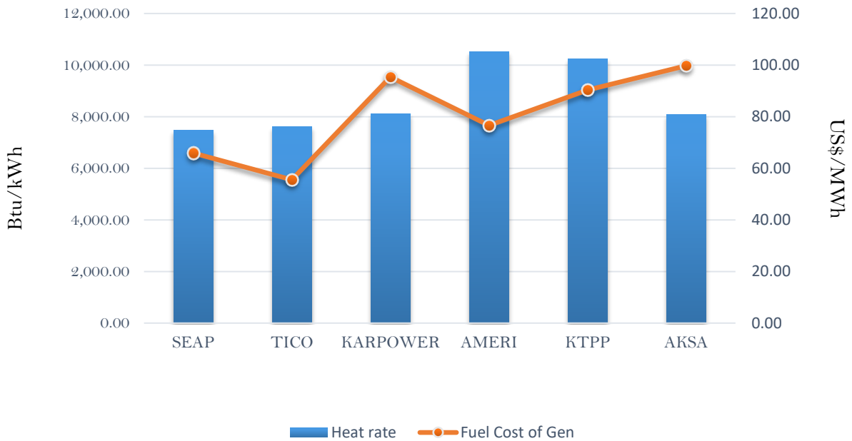
Efficiency and fuel cost of generation on the 6th October 2018
