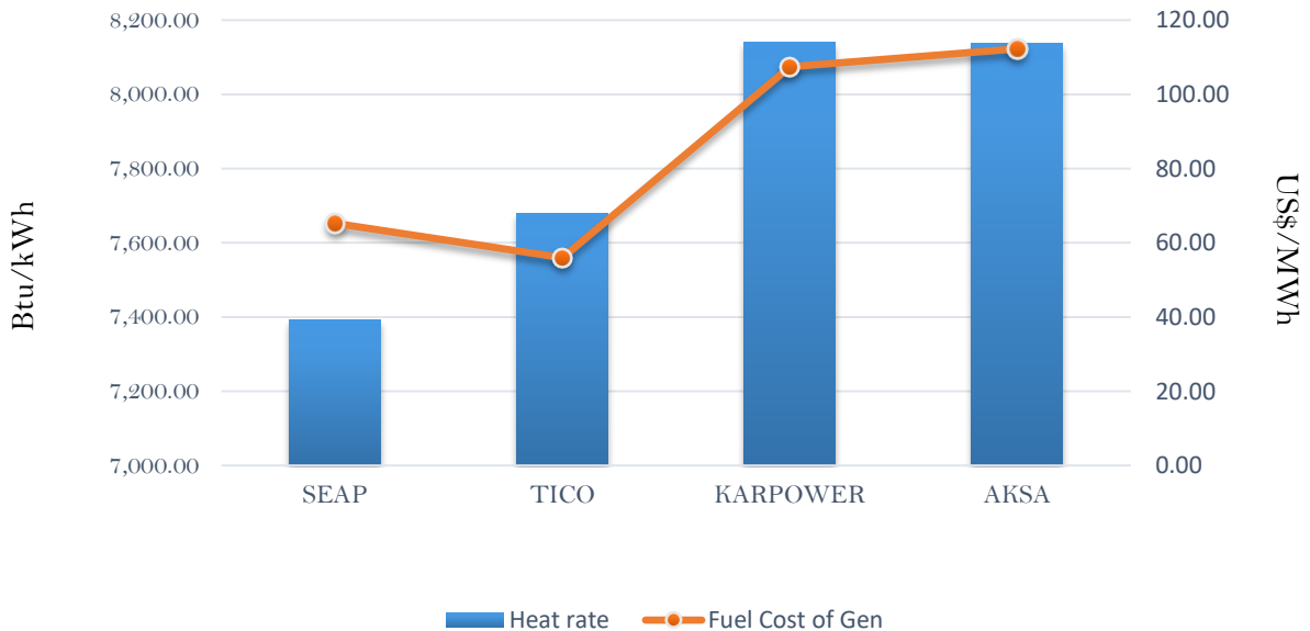
Efficiency and fuel cost of generation on the 2nd October 2018
