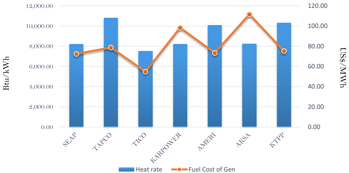
Efficiency and fuel cost of generation on the 2nd November 2018
