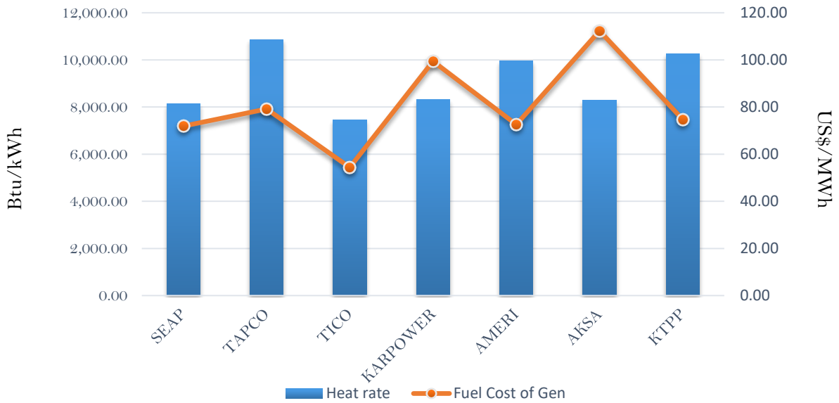
Efficiency and fuel cost of generation on the 1st November 2018
