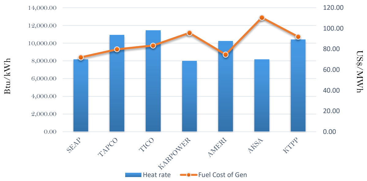
Efficiency and fuel cost of generation on the 5th November 2018
