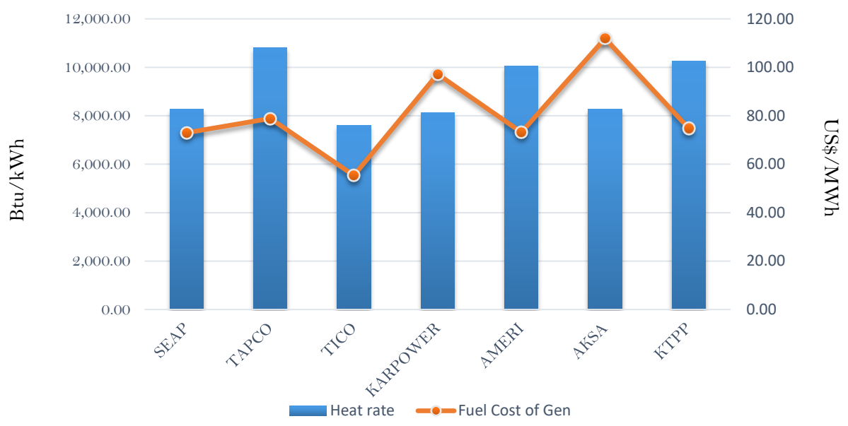
Efficiency and fuel cost of generation on the 3rd November 2018
