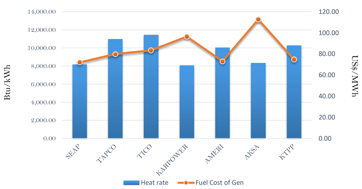
Efficiency and fuel cost of generation on the 4th November 2018
