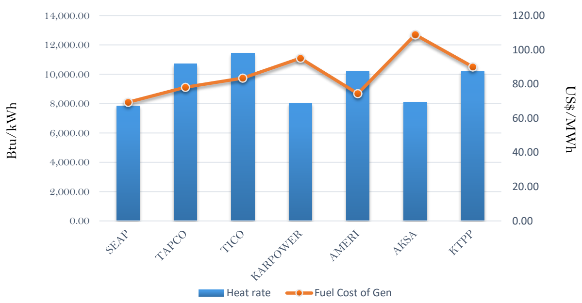
Efficiency and fuel cost of generation on the 6th November 2018
