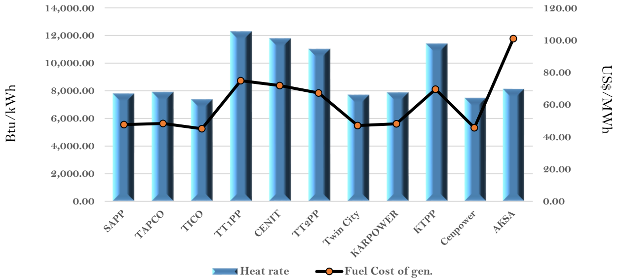
Efficiency and fuel cost of generation on the 13th May 2021
