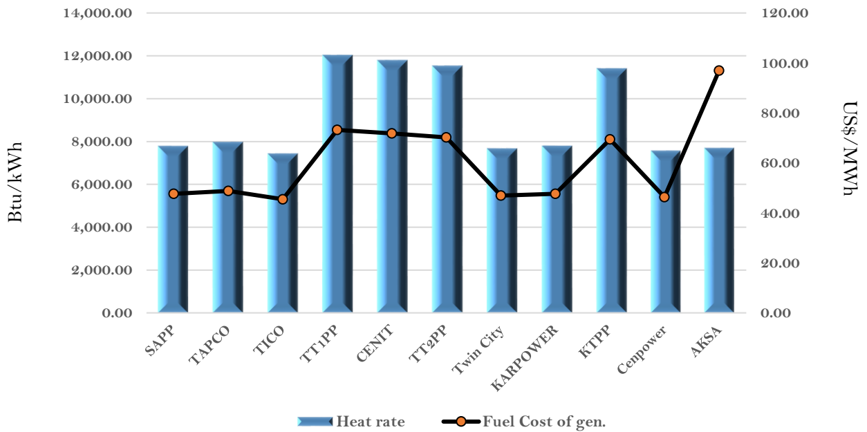
Efficiency and fuel cost of generation on the 14th May 2021
