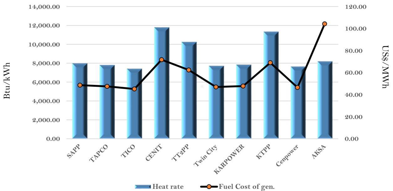
Efficiency and fuel cost of generation on the 7th May 2021
