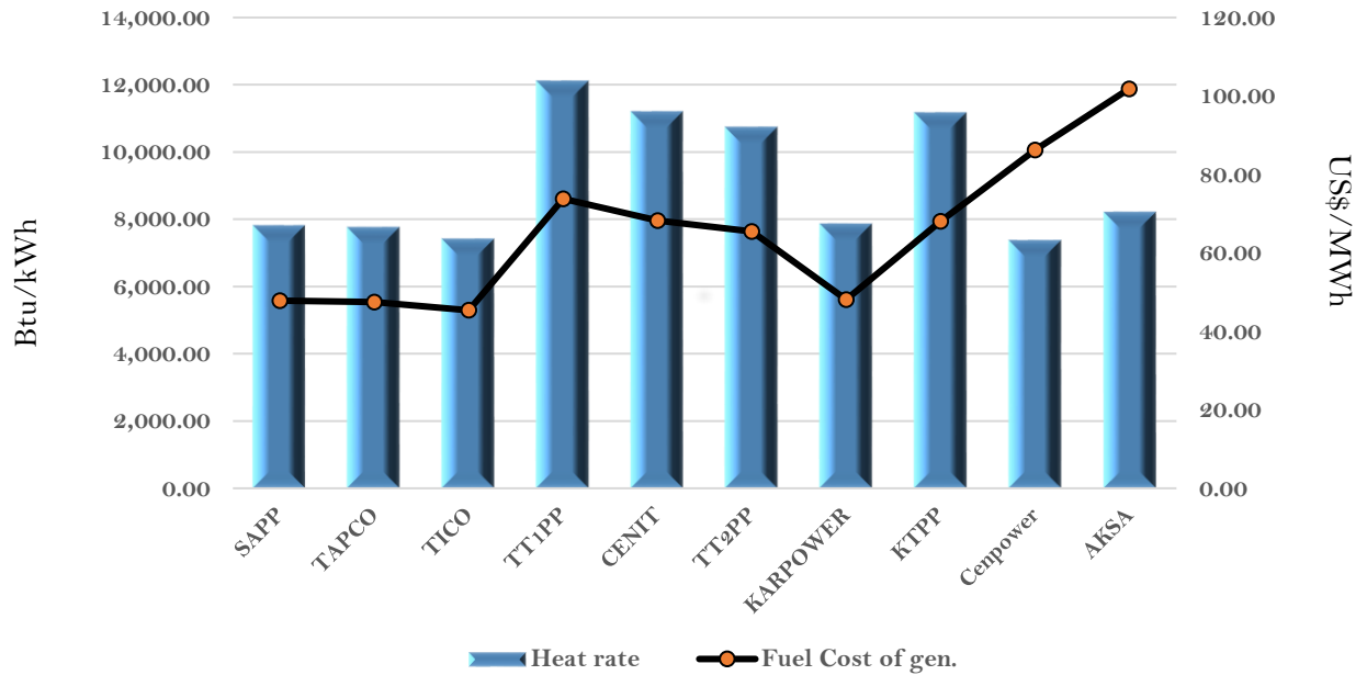
Efficiency and fuel cost of generation on the 19th March 2021
