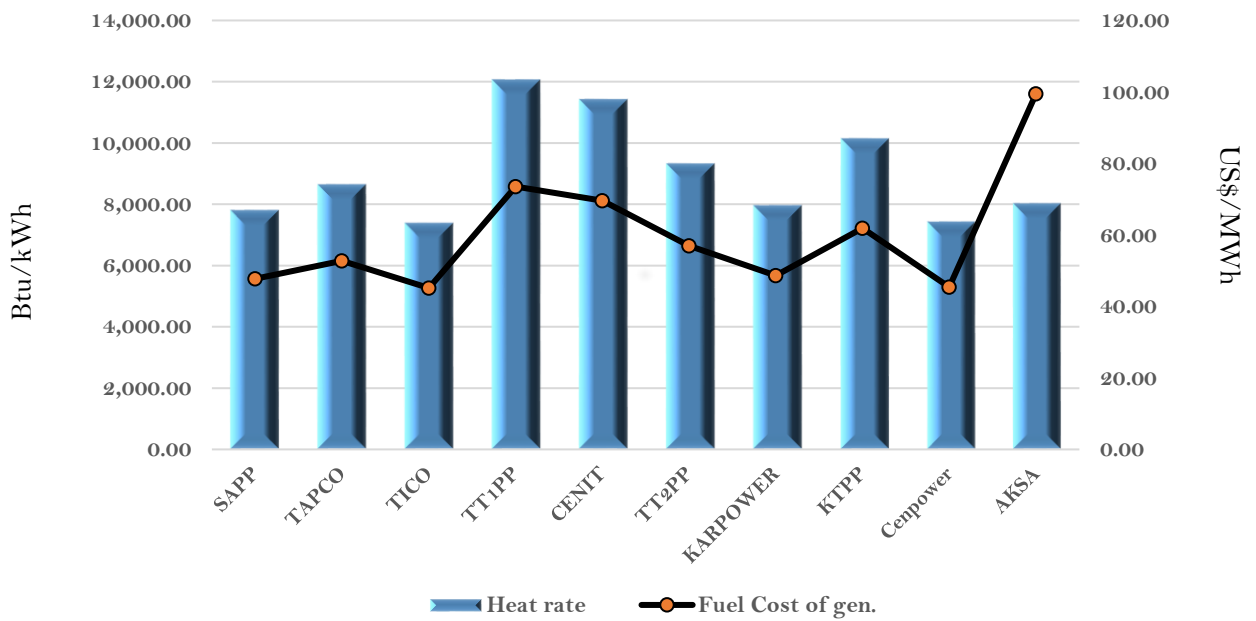
Efficiency and fuel cost of generation on the 21st March 2021
