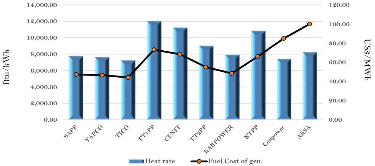
Efficiency and fuel cost of generation on the 18th March 2021
