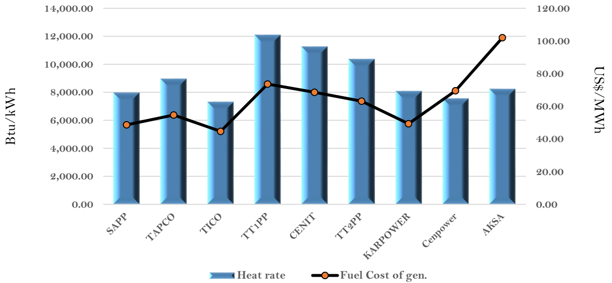
Efficiency and fuel cost of generation on the 20th March 2021
