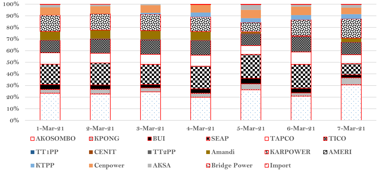
Shares of power plant generation
