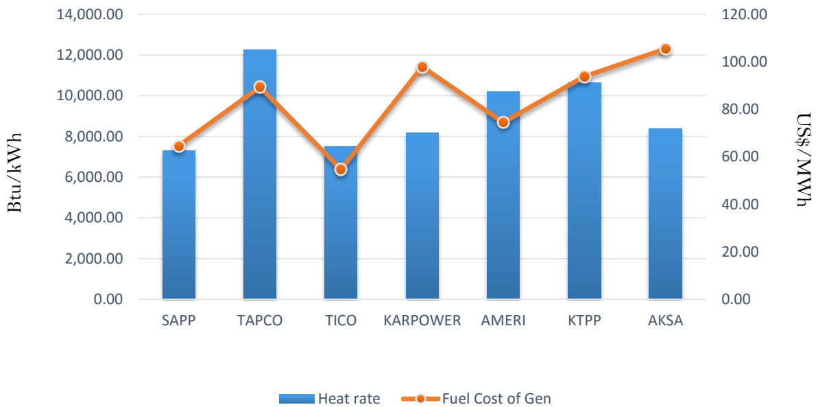
Efficiency and fuel cost of generation on the 23rd June 2018
