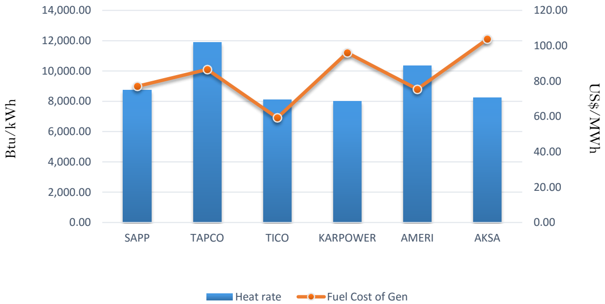
Efficiency and fuel cost of generation on the 22nd June 2018
