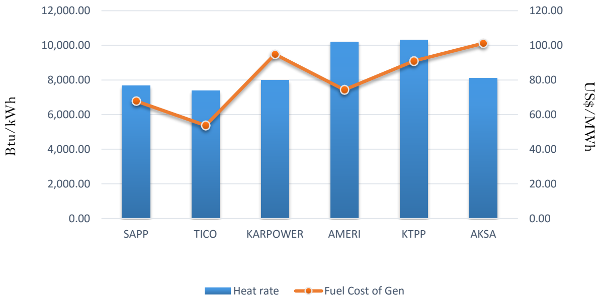
Efficiency and fuel cost of generation on the 25th June 2018
