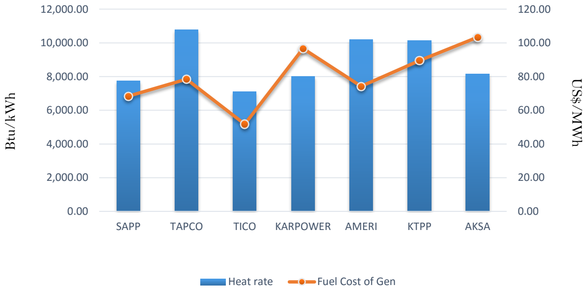
Efficiency and fuel cost of generation on the 26th June 2018
