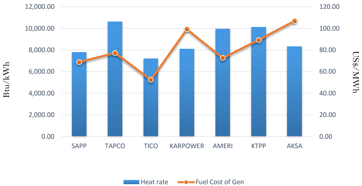
Efficiency and fuel cost of generation on the 27th June 2018
