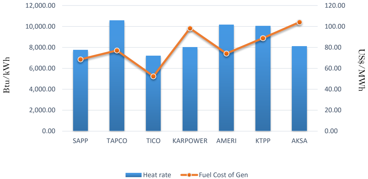
Efficiency and fuel cost of generation on the 28th June 2018
