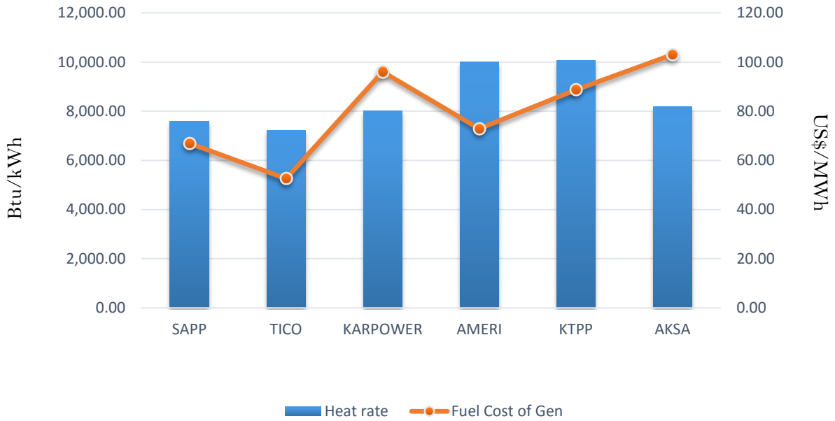
Efficiency and fuel cost of generation on the 24th June 2018
