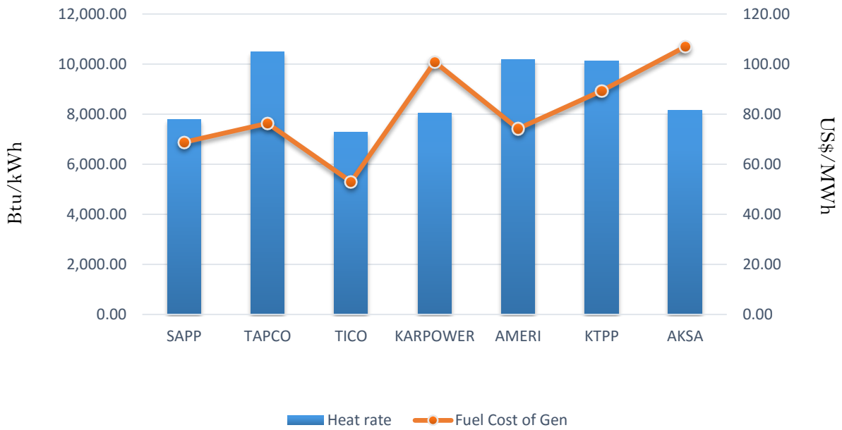
Efficiency and fuel cost of generation on the 29th June 2018
