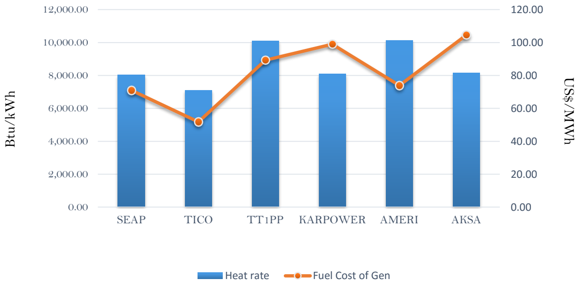
Efficiency and fuel cost of generation on the 27th July 2018
