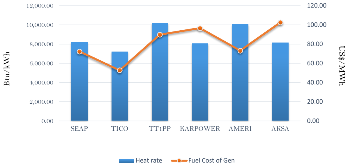
Efficiency and fuel cost of generation on the 31st July 2018
