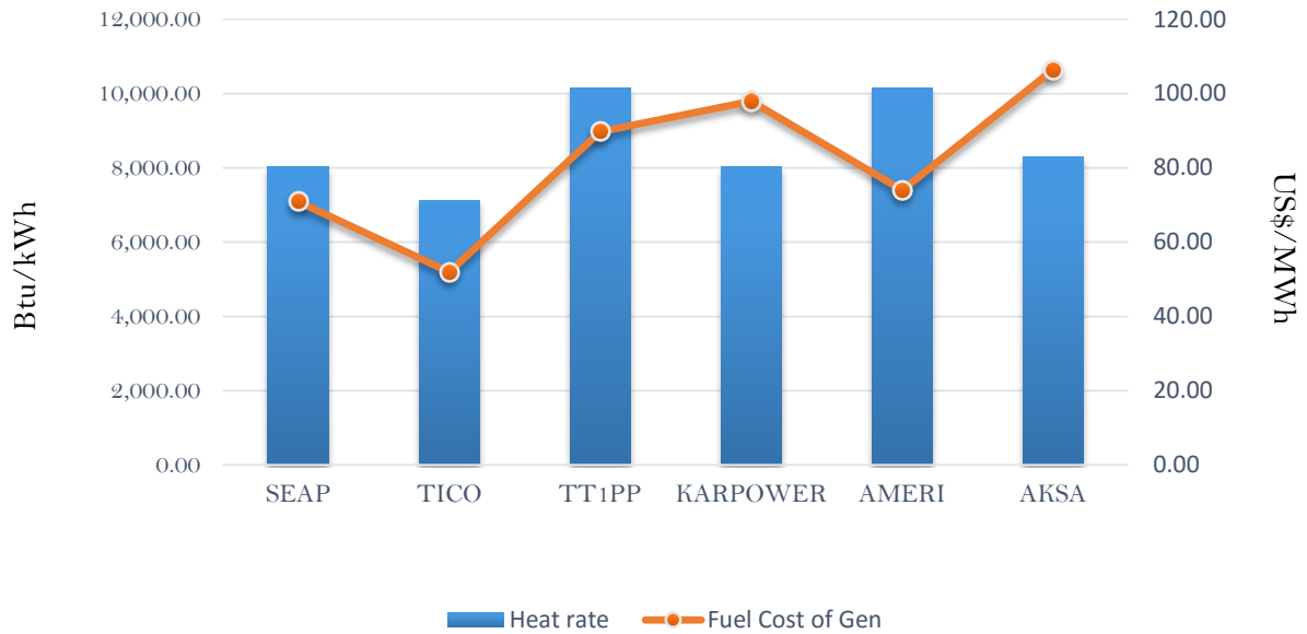
Efficiency and fuel cost of generation on the 28th July 2018
