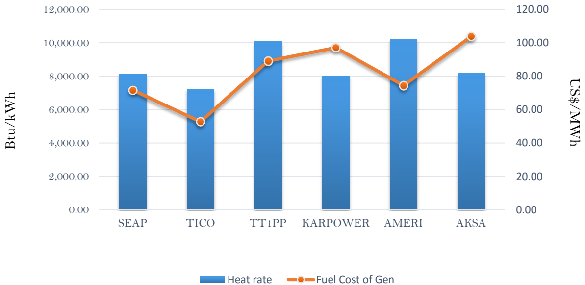
Efficiency and fuel cost of generation on the 25th July 2018
