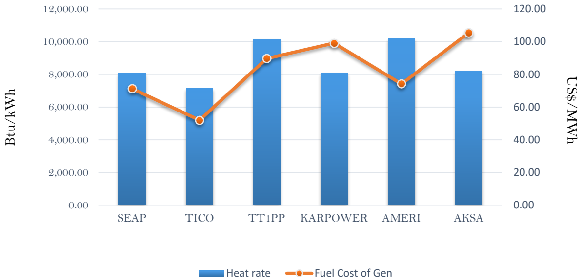
Efficiency and fuel cost of generation on the 26th July 2018
