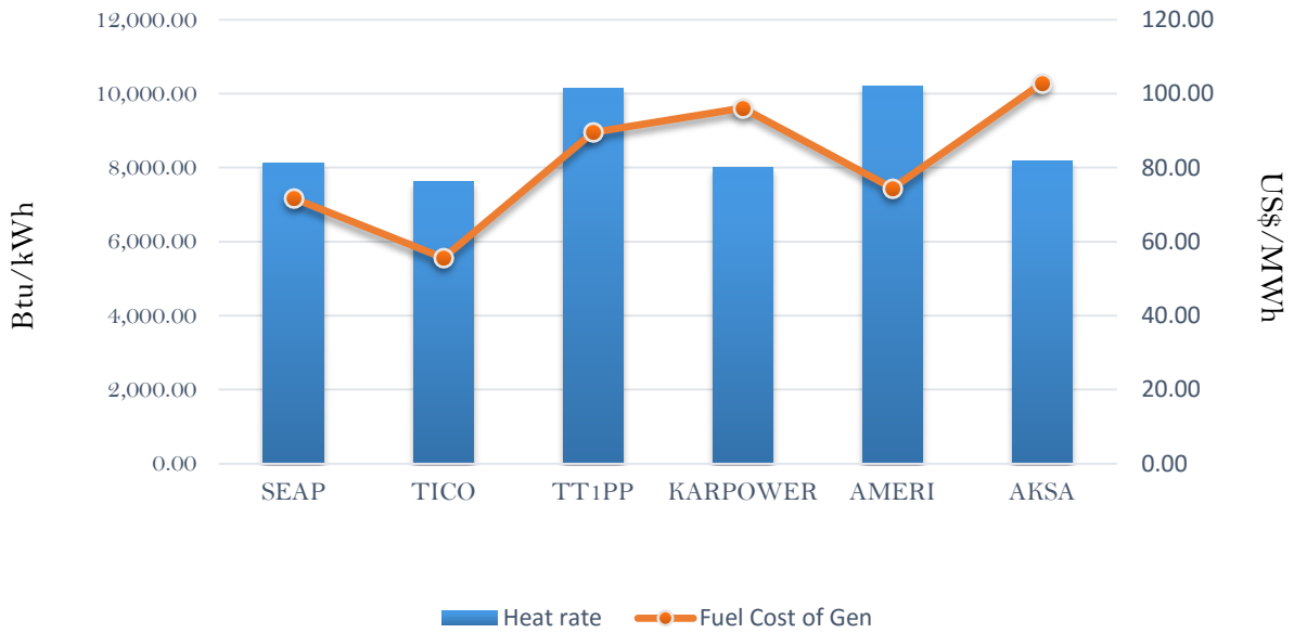
Efficiency and fuel cost of generation on the 24th July 2018
