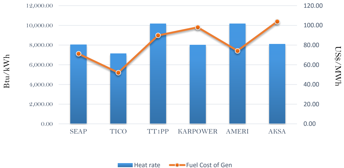
Efficiency and fuel cost of generation on the 29th July 2018
