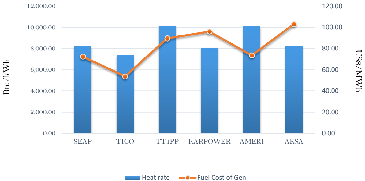
Efficiency and fuel cost of generation on the 22nd July 2018
