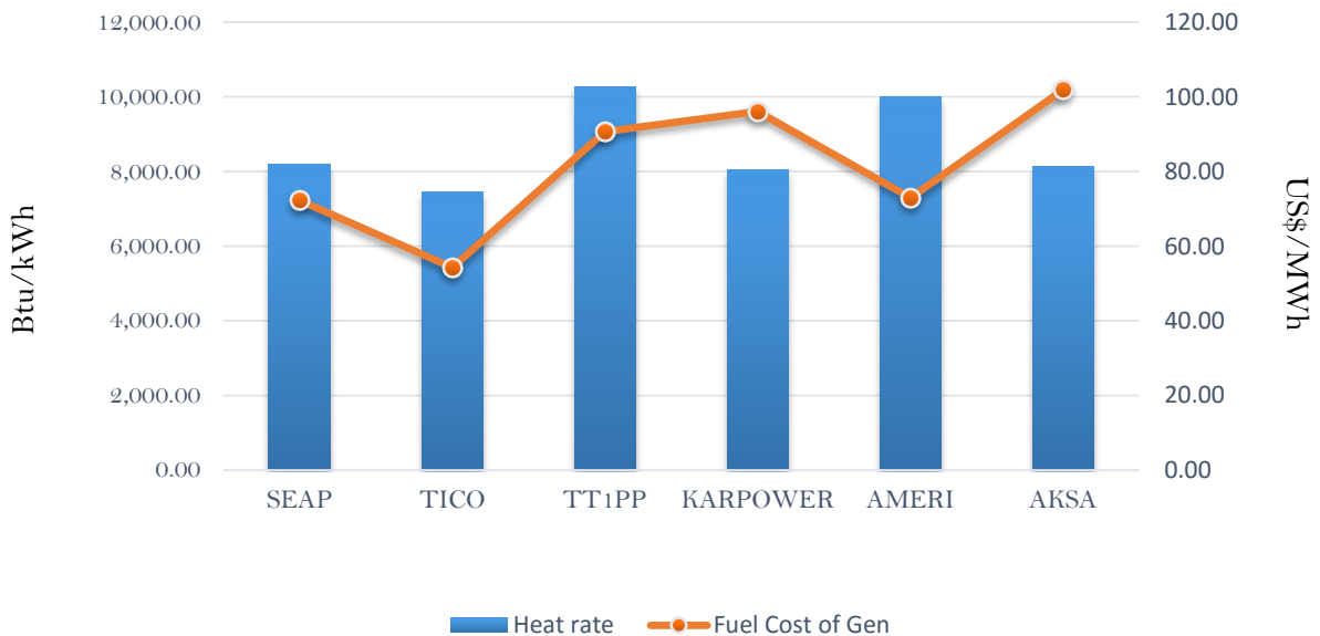
Efficiency and fuel cost of generation on the 23rd July 2018
