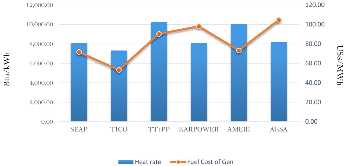
Efficiency and fuel cost of generation on the 30th July 2018
