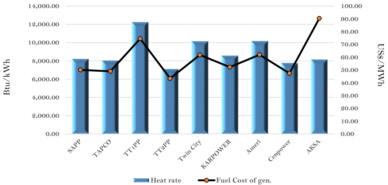
Efficiency and fuel cost of generation on the 21st January 2021
