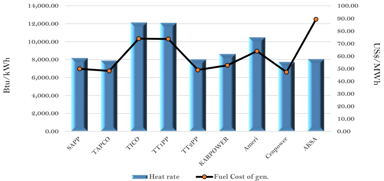
Efficiency and fuel cost of generation on the 20th January 2021
