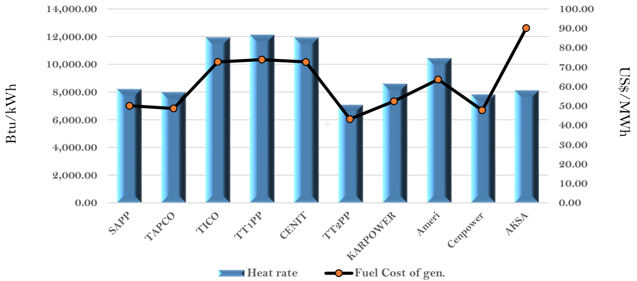
Efficiency and fuel cost of generation on the 13th January 2021
