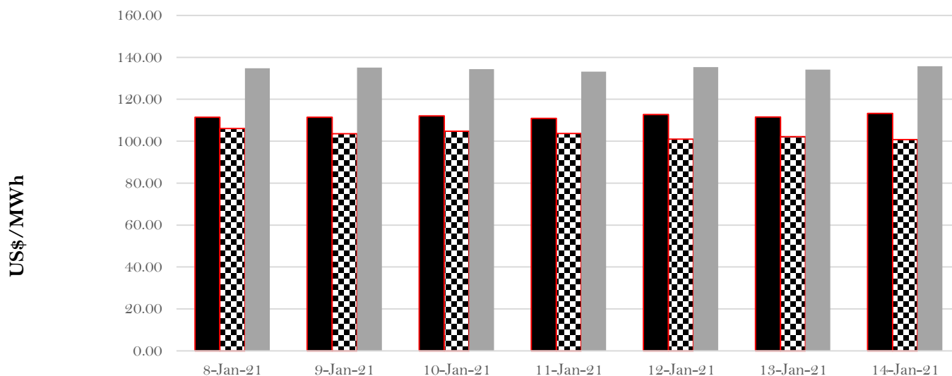
System Marginal Cost Vs Average Market Prices for Week 2 of January 2021
