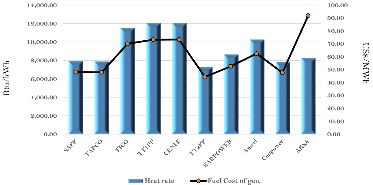
Efficiency and fuel cost of generation on the 14th January 2021
