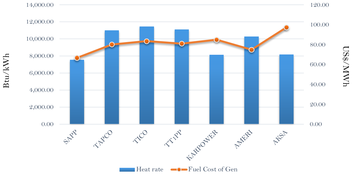
Efficiency and fuel cost of generation on the 31st January 2019
