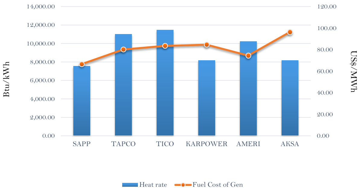
Efficiency and fuel cost of generation on the 29th January 2019
