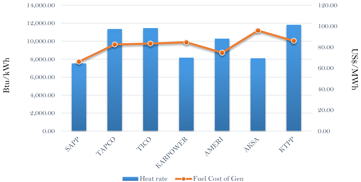
Efficiency and fuel cost of generation on the 25th January 2019
