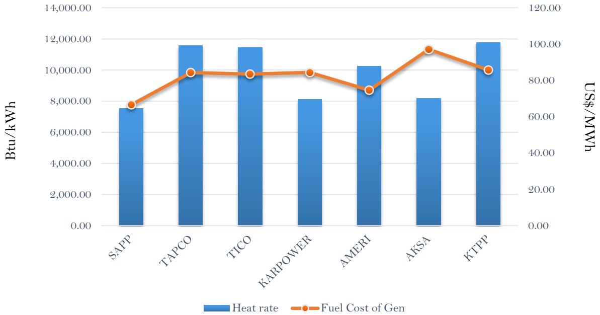
Efficiency and fuel cost of generation on the 27th January 2019
