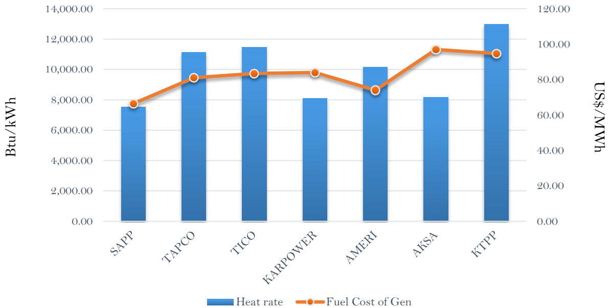
Efficiency and fuel cost of generation on the 27th January 2019
