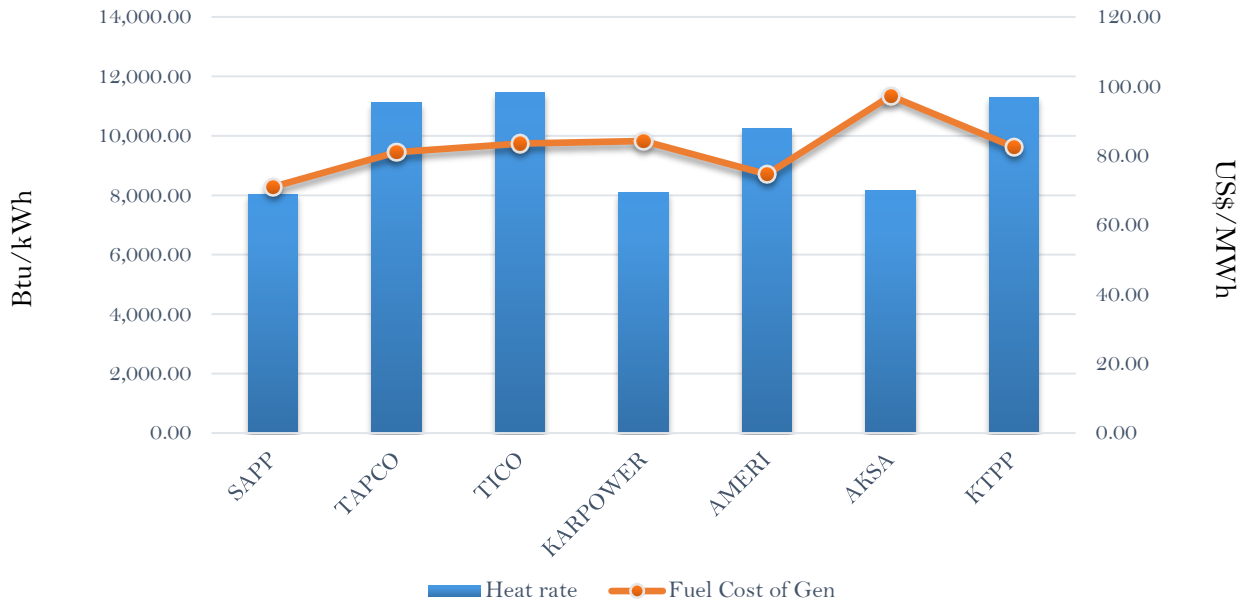
Efficiency and fuel cost of generation on the 23rd January 2019
