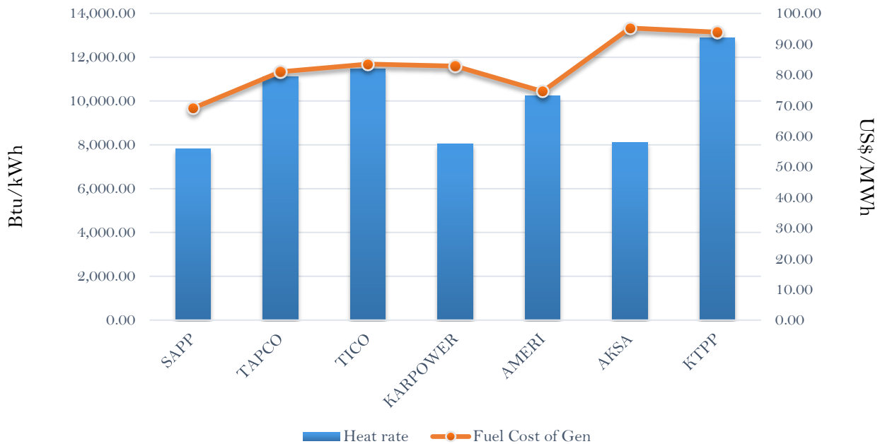
Efficiency and fuel cost of generation on the 23rd January 2019
