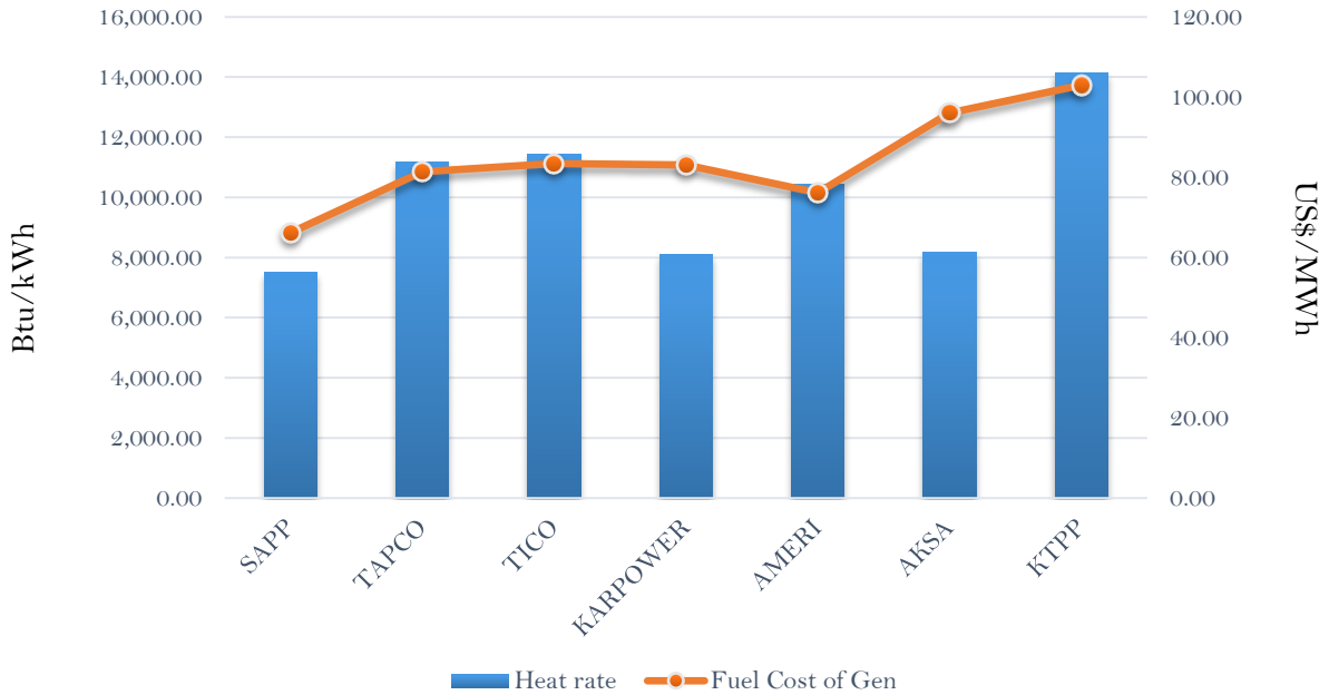
Efficiency and fuel cost of generation on the 25th January 2019
