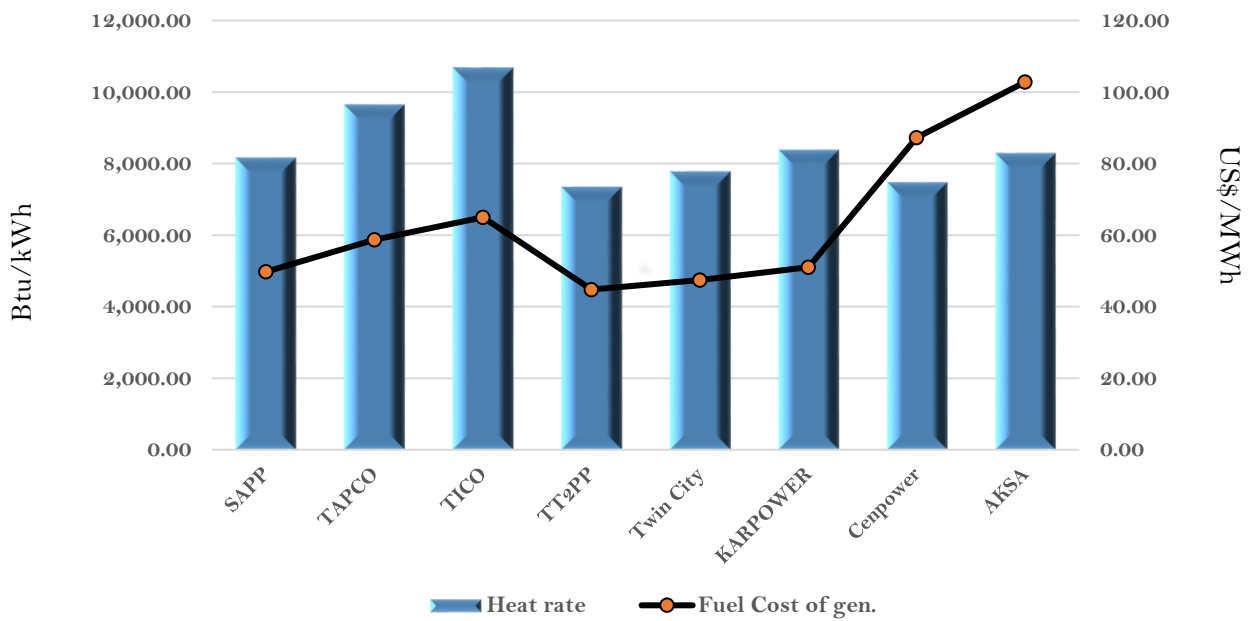
Efficiency and fuel cost of generation on the 28th February 2021
