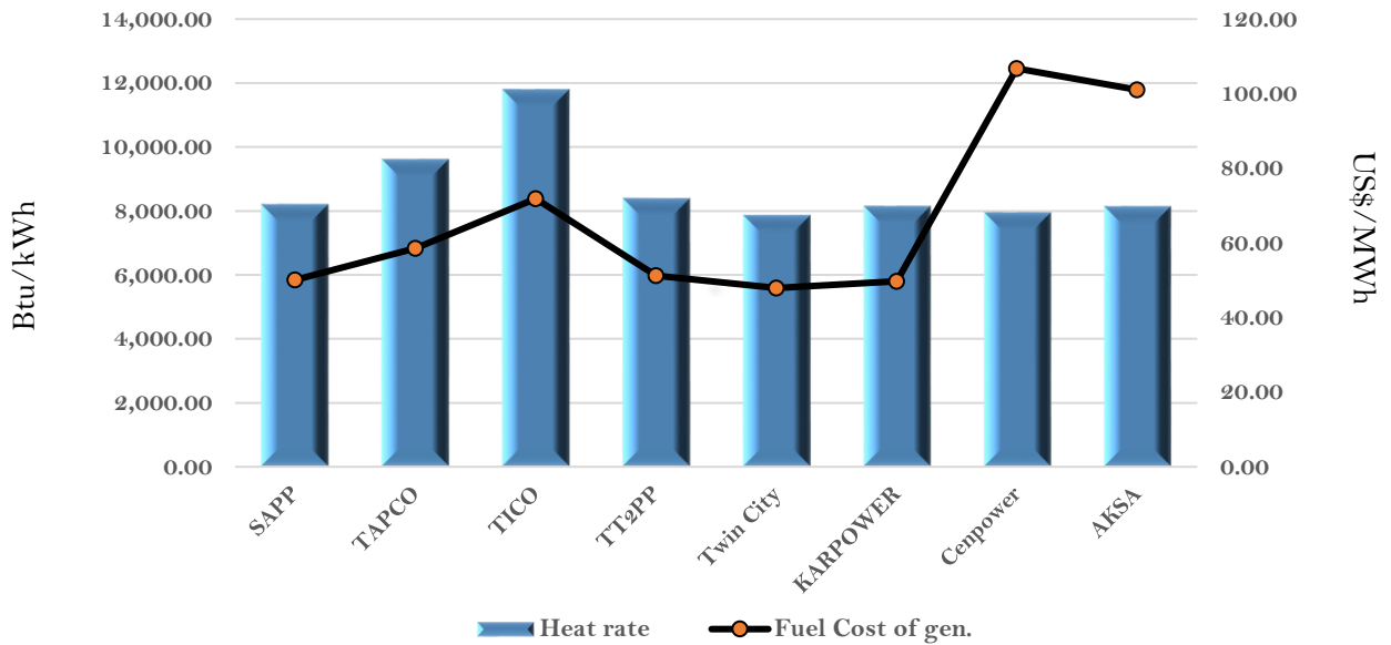
Efficiency and fuel cost of generation on the 27th February 2021
