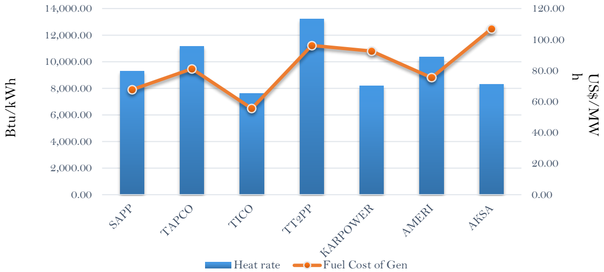
Efficiency and fuel cost of generation on the 28th February 2019
