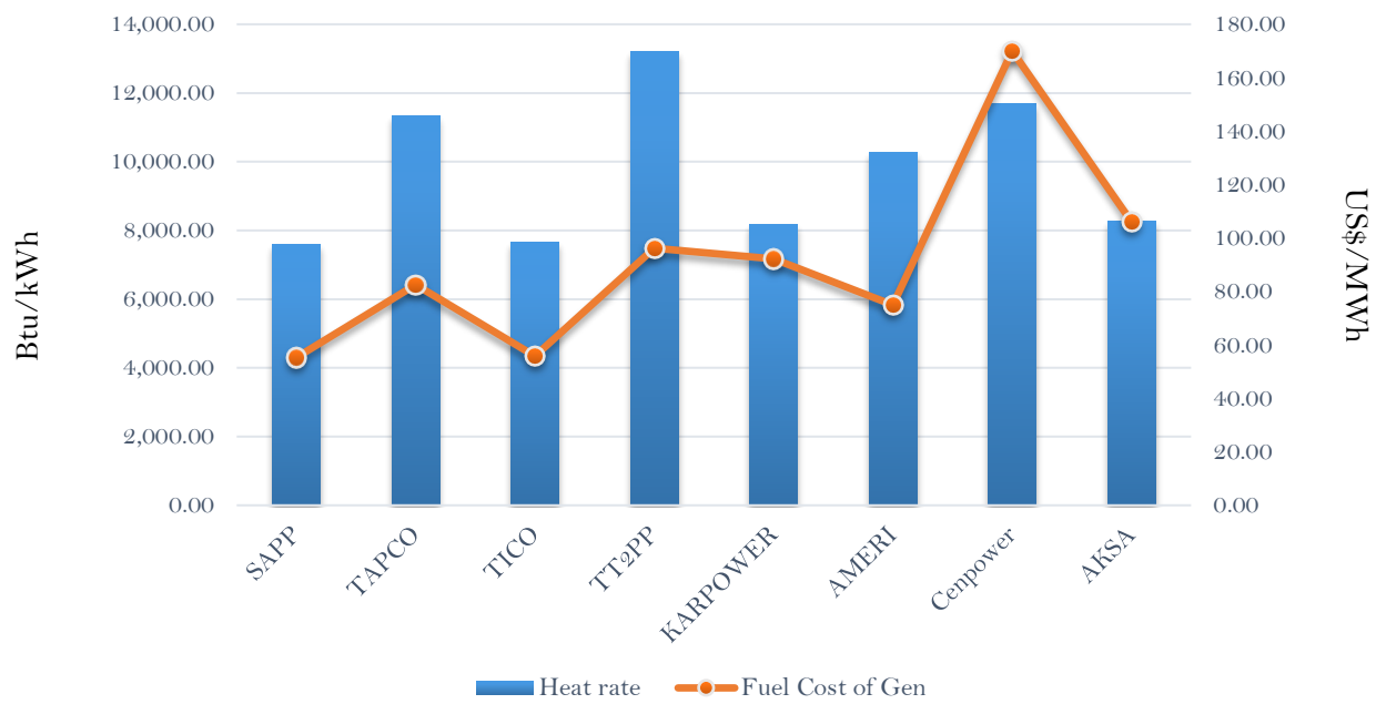
Efficiency and fuel cost of generation on the 23rd February 2019
