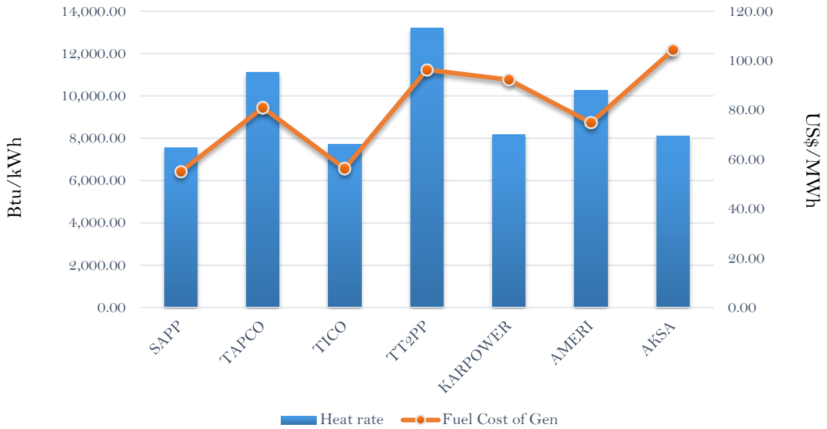
Efficiency and fuel cost of generation on the 25th February 2019
