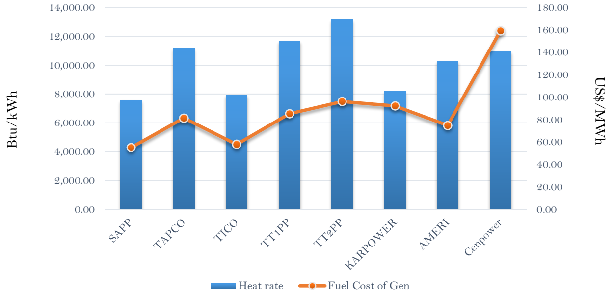
Efficiency and fuel cost of generation on the 23rd February 2019
