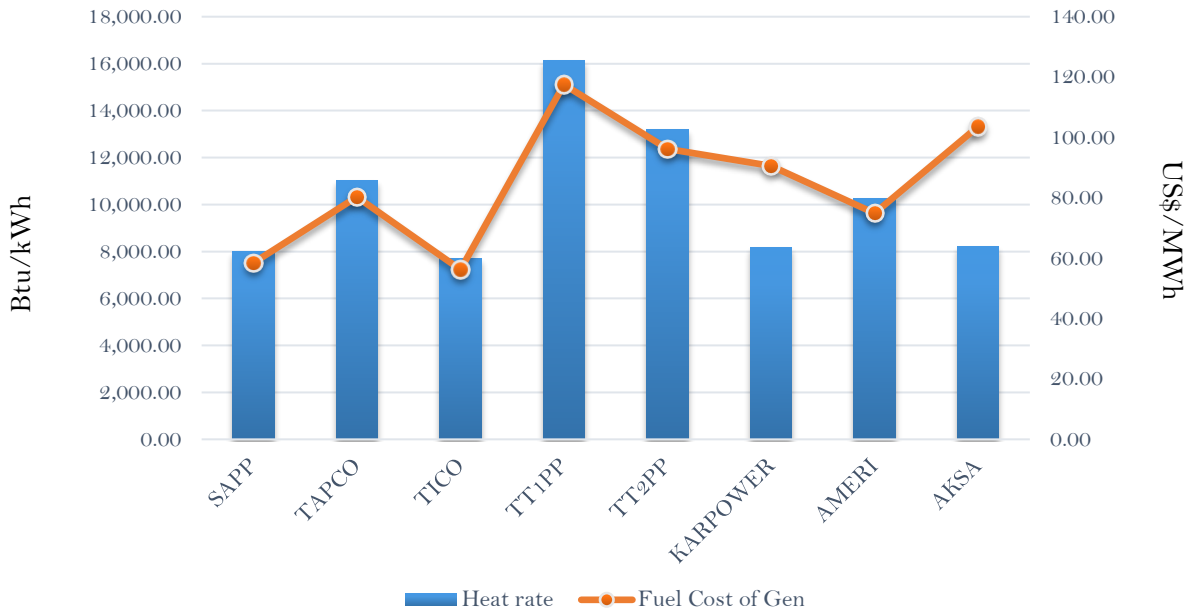
Efficiency and fuel cost of generation on the 27th February 2019
